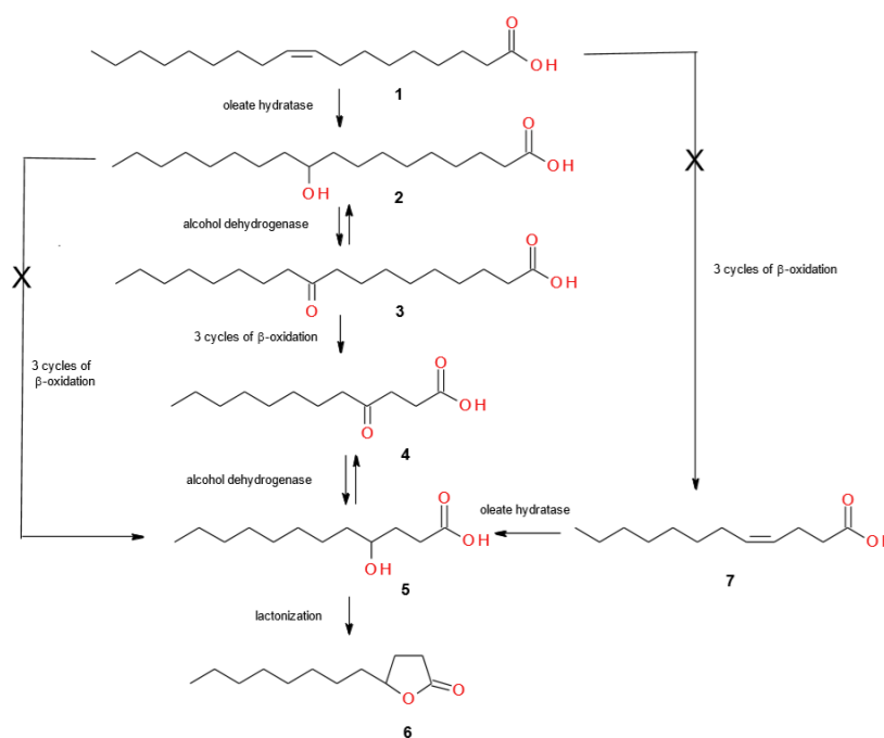
Scheme 1. Pathways of oleic acid (1) biotransformations.
