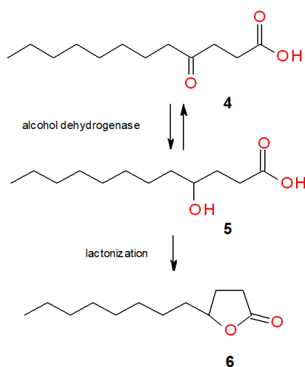
Scheme 2. Reduction of 4-ketolauric acid (4) with following cyclization to \gamma -dodecalactone (6).
