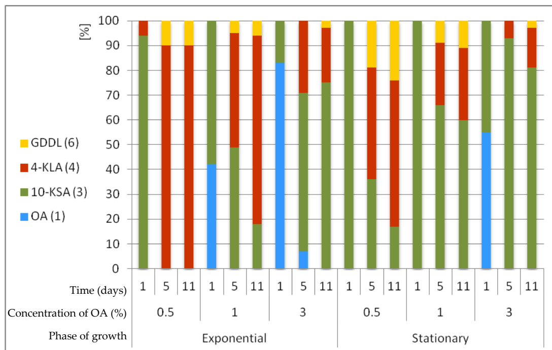
Figure 1. Effect of Micrococcus luteus PCM525 growth phase and concentration of substrate on transformation of oleic acid ( 1 ) (in % according to GC–MS).
