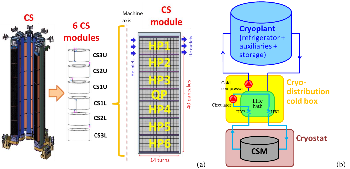
Figure 2 (a) Sketch of the ITER CS and its subcomponents (U = upper, L = lower, HP = hexa-pancake, QP = quad-pancake), partially taken from (Libeyre et al., 2015); (b) scheme of the facility for the CSM cold tests taken as reference in the present work.
