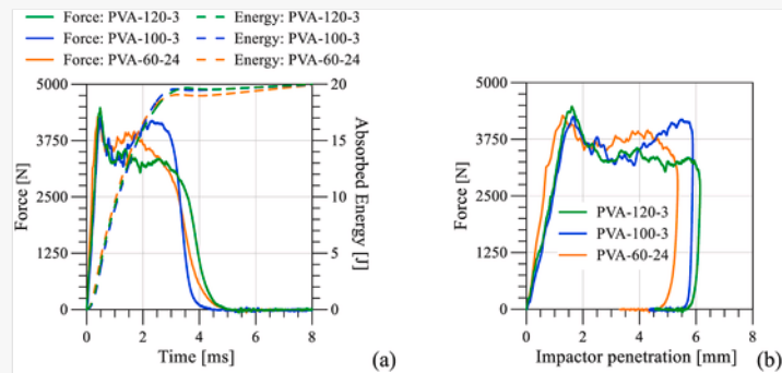
Impact tests reinforced materials, 20 J: representative curves (a) force and energy vs. time; (b) force vs. impactor penetration.
