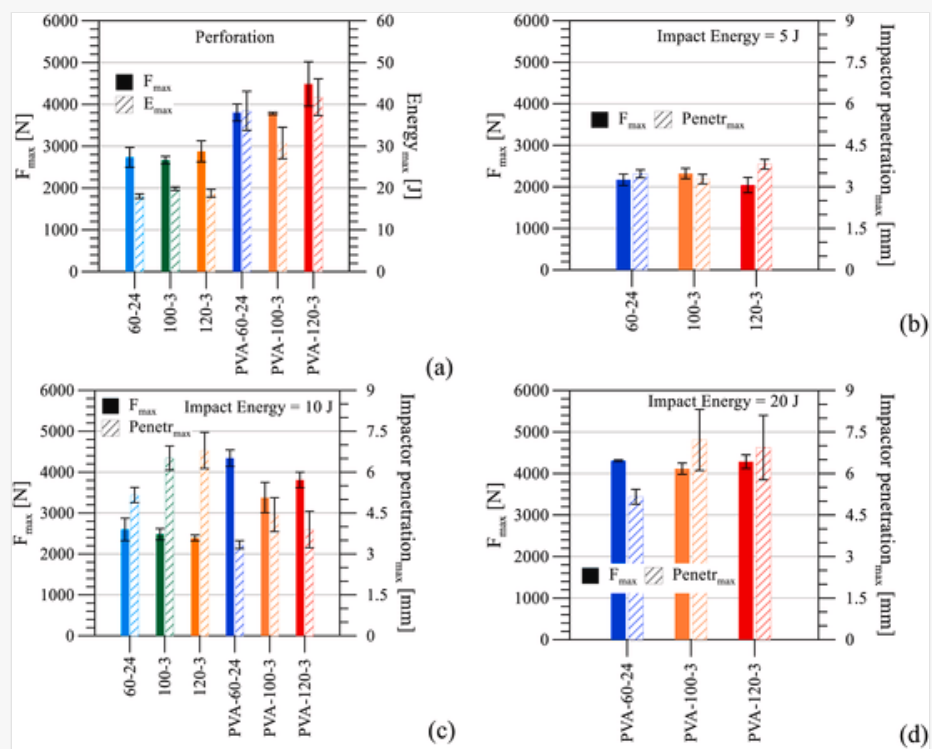
Impact tests comparison at: (a) perforation; (b) impact energy 5 J; (c) impact energy 10 J; (d) impact energy 20 J. Average and standard deviation (error bar) of three measurements.
