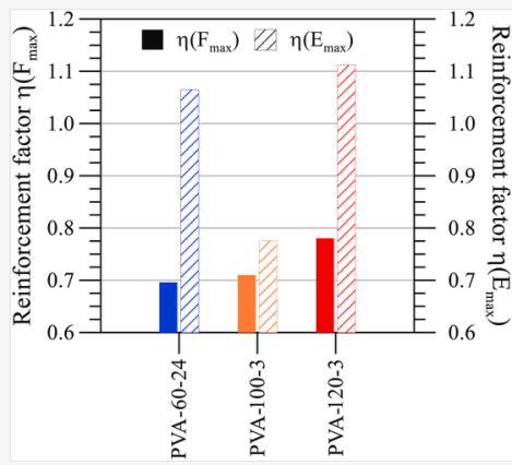
Impact tests at perforation: reinforcement factor for the maximum force and absorbed energy.
