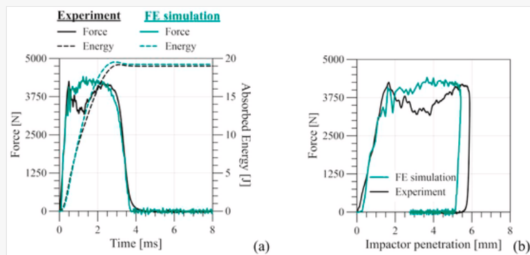
Comparison of experimental and numerical results for material PVA-100-3: (a) force and energy vs. time; (b) force vs. impactor penetration.
