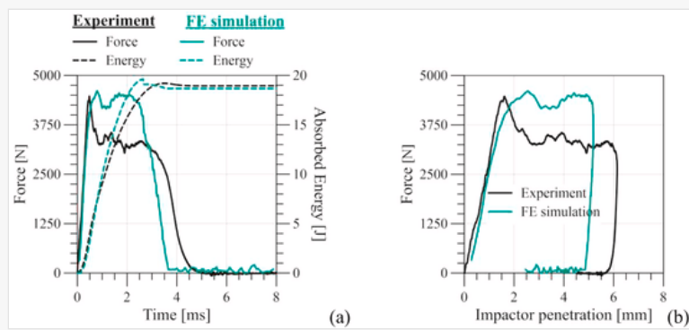
Comparison of experimental and numerical results for material PVA-120-3: (a) force and energy vs. time; (b) force vs. impactor penetration.
