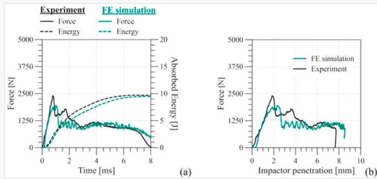
Comparison of experimental and numerical results for material 120-3: (a) force and energy vs. time; (b) force vs. impactor penetration.
