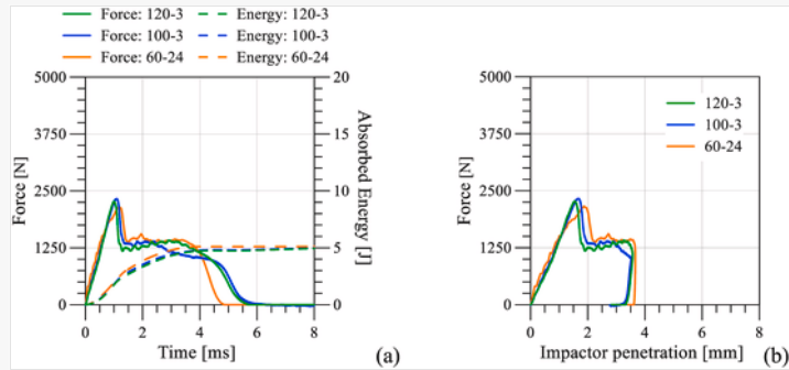
Impact tests of plain materials, 5 J: representative curves (a) force and energy vs. time; (b) force vs. impactor penetration.
