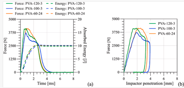
Impact tests of reinforced materials, 10 J: representative curves (a) force and energy vs. time; (b) force vs. impactor penetration.
