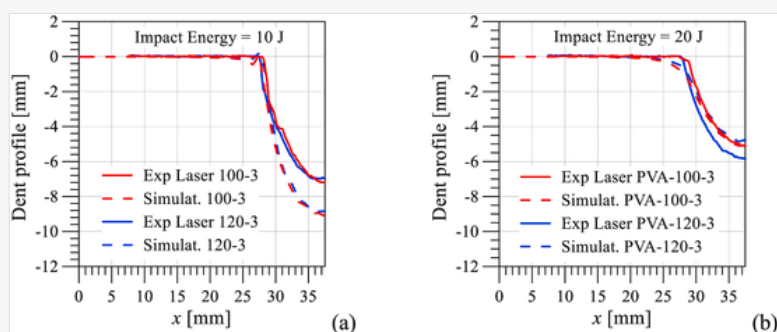
Comparison of representative experimental and numerical results of the impact surface profile along one line of symmetry: (a) unreinforced materials 100-3 and 120-3, impact energy 10 J; (b) reinforced materials PVA-100-3 and PVA-120-3 impact energy 20 J.
