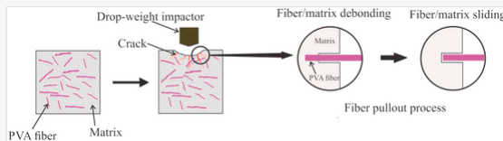
Sketch of the role of PVA fiber in enhancing the impact resistance of the hot-pressed reinforced composite via crack growth resistance.
