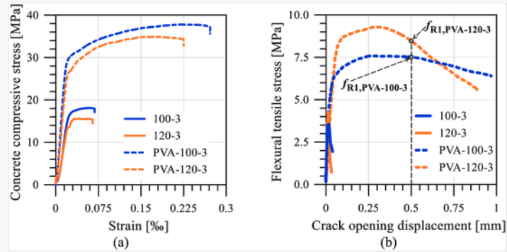
Experimental (a) compressive stress-strain, (b) flexural tensile stress vs. crack opening displacement (COD) curves.
