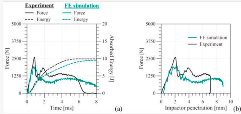
Comparison of experimental and numerical results for material 100-3: (a) force and energy vs. time; (b) force vs. impactor penetration.
