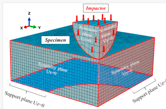
FE mesh and boundary conditions of the impactor and the specimen.
