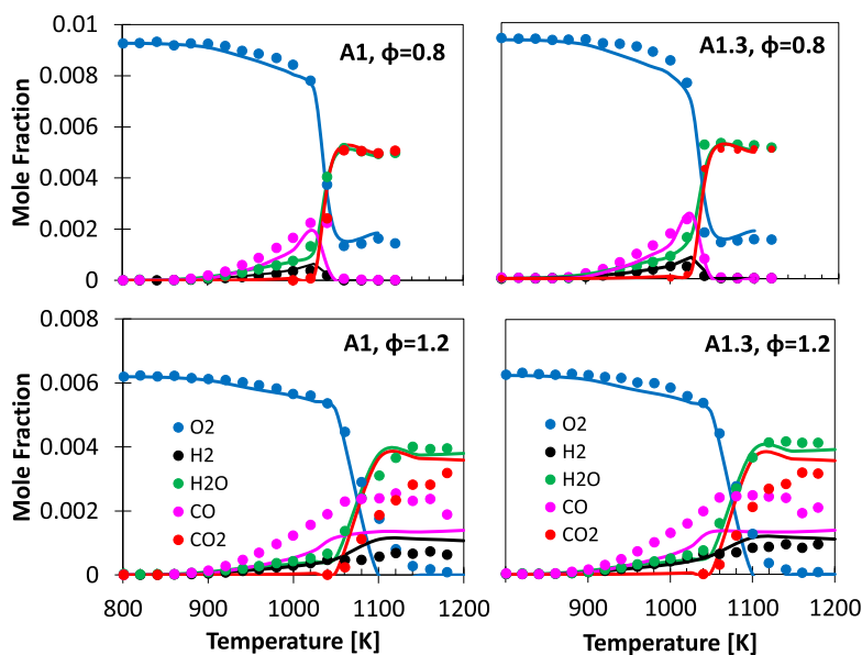
Fig. 1. Major species profiles ( \text{H}_2 , \text{H}_2\text{O} , \text{O}_2 , \text{CO}_2 , \text{CO} ) measurement (Symbols) and simulation (Lines). Left panels: A1, \varphi = 0.8 (top), \varphi = 1.2 (bottom). Right panels: A1.3, \varphi = 0.8 (top), \varphi = 1.2 (bottom).
