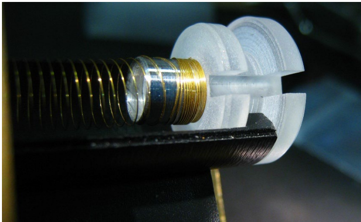
Figure 1. - A detail of the avalanche confinement TEPC. The gold-plated tungsten helix, 6 mm in diameter, and the Rexolite cap with the 1 mm slit for the passage of accelerated light ions or alpha particles from an external source.
