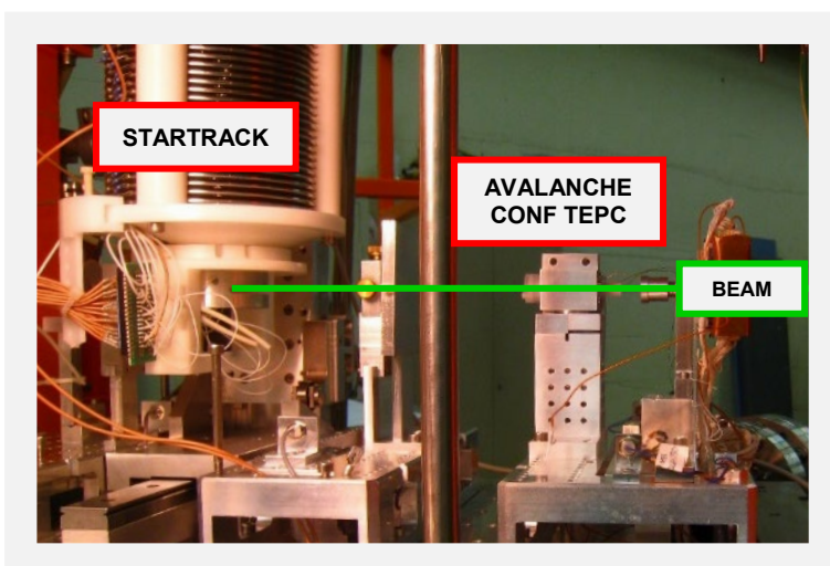
Figure 2. - A picture of the measuring set-up: the primary particle impinges on both detectors, the Startrack counter and the avalanche-confinement TEPC, for first systematic microdosimetry and nanodosimetry comparison.
