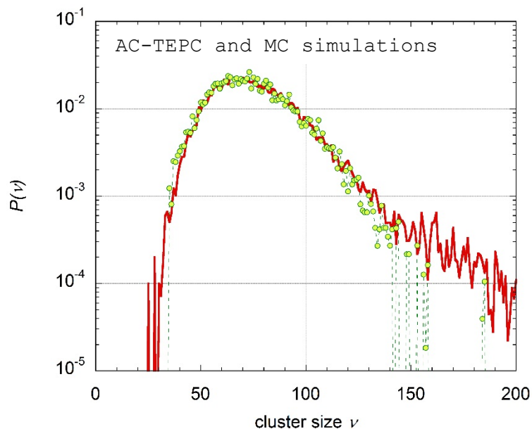
Figure 3. - The cluster size probability P(\nu) measured with the avalanche-confinement TEPC at 25 nm (symbols connected by a slash line), and the corresponding results of Monte Carlo simulations (continuous line).
