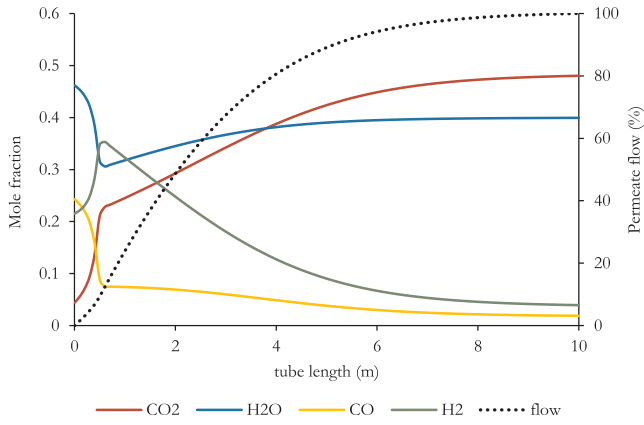
Fig. 4. Retentate composition profile and permeate flow in % for a tube length of the MAWGS reactor for a case designed for maximum hydrogen recovery.
