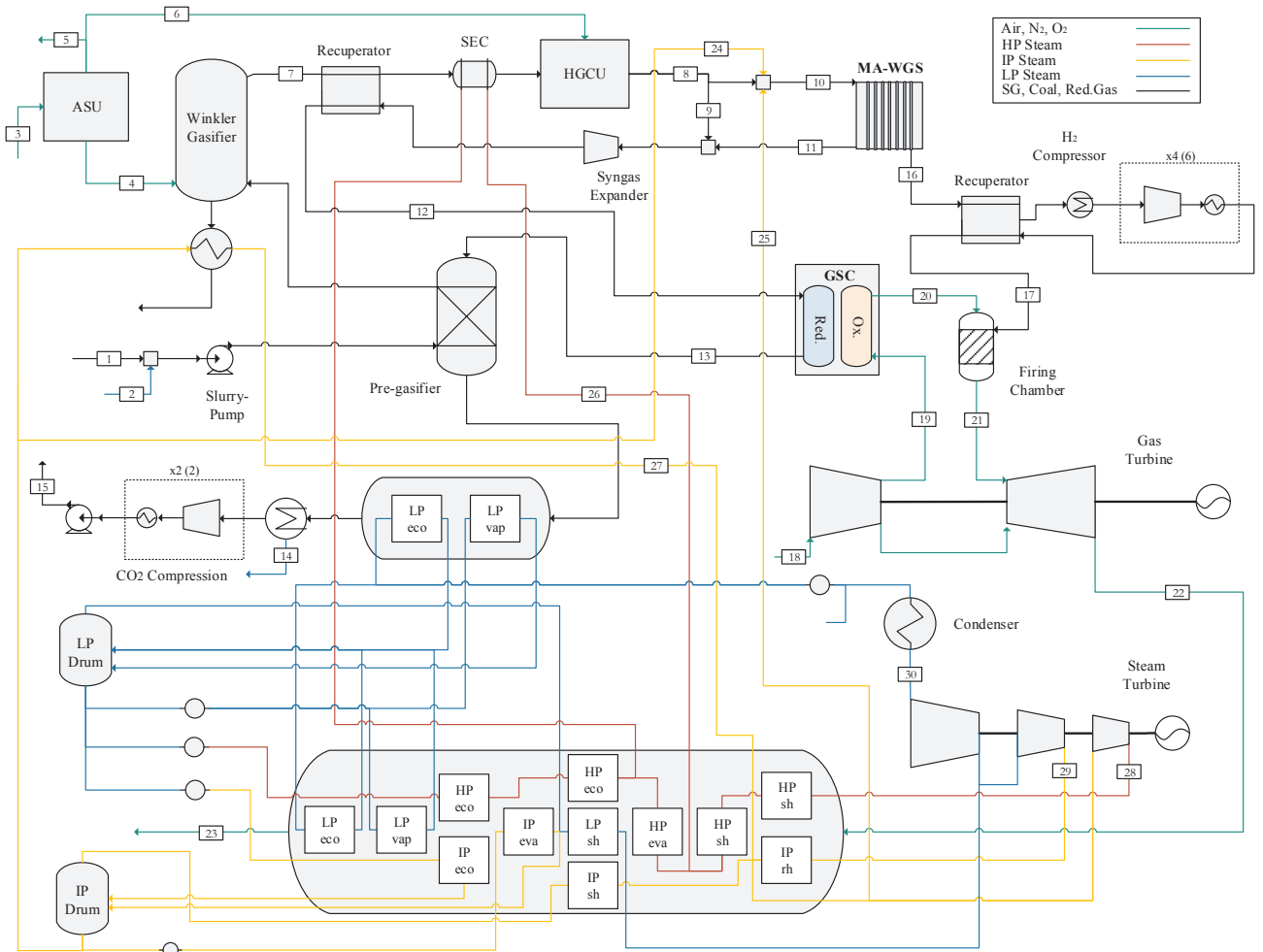
Fig. 8. Schematic of the GSC-MAWGS IGCC power plant with slurry pre-gasification. Stream data can be found in Table 10 in the Appendix.
