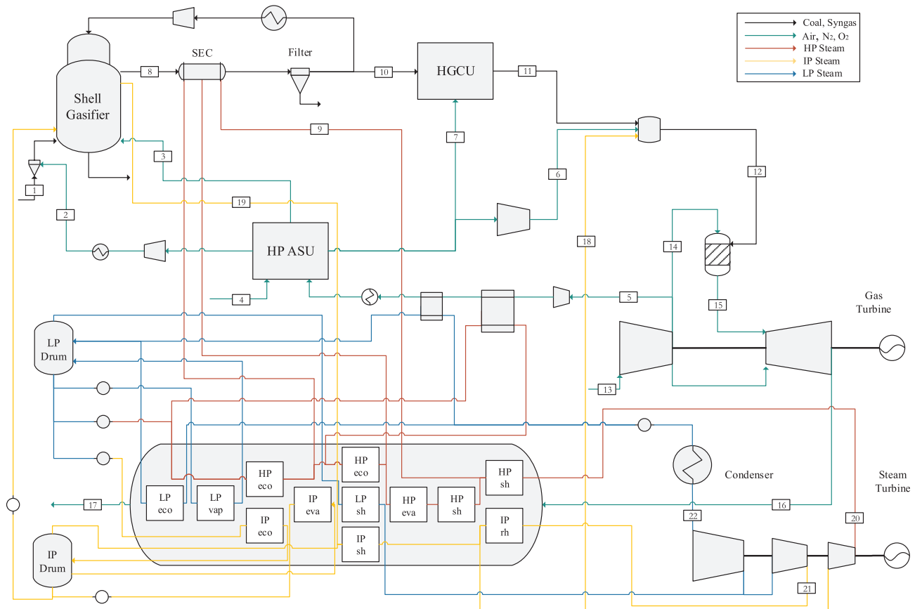
Fig. 5. Schematic of the Unabated IGCC power plant. Stream data can be found in Table 7 in the Appendix.
