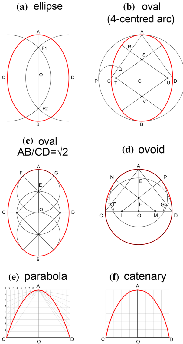
Fig. 4 The array of the curves taken into account: a ellipse; b , c oval; d ovoid; e parabola; f catenary (drawing by F. Fiorillo)
