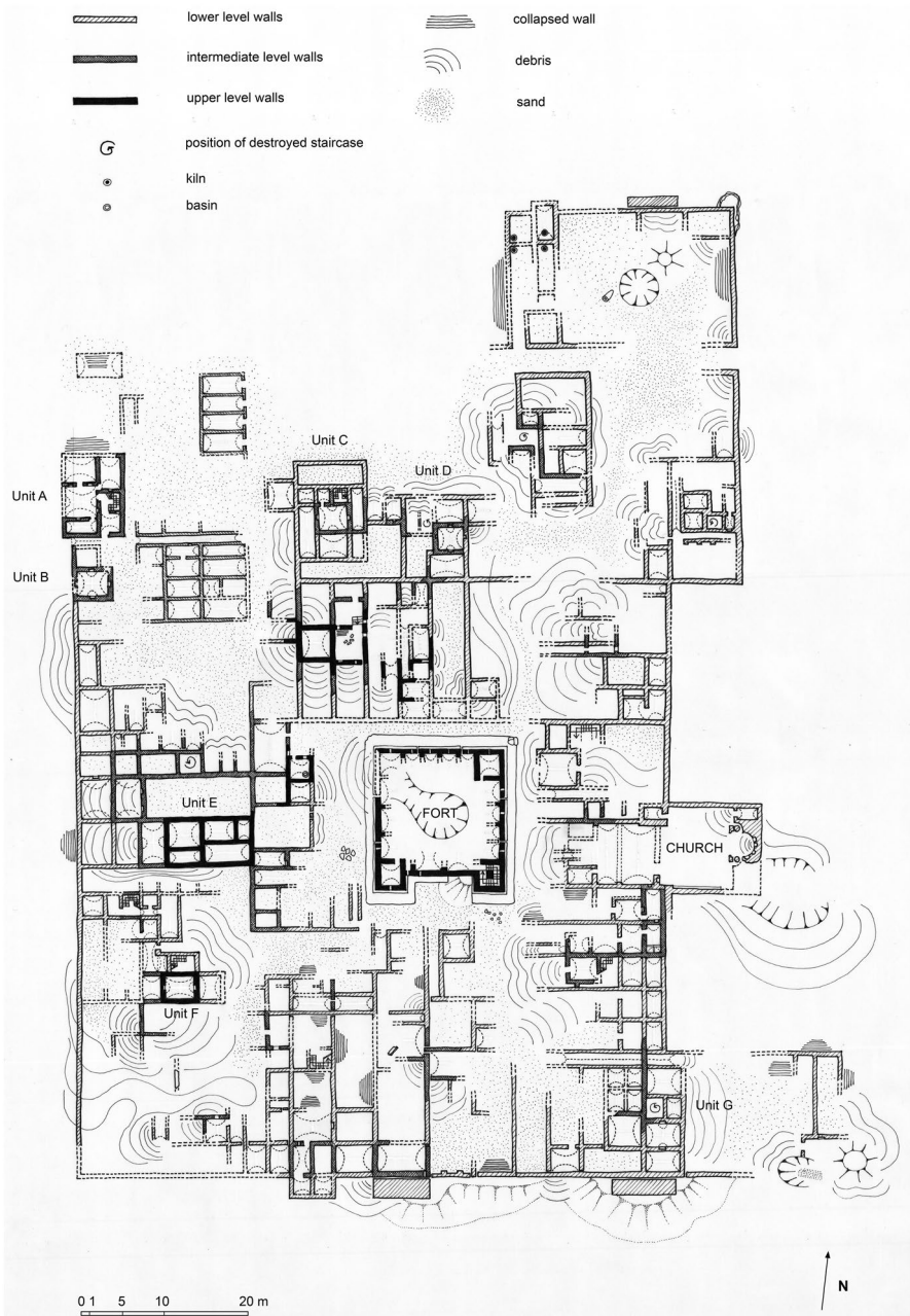
Fig. 5 Plan of the fortified settlement of Umm al-Dabadib (drawing by C. Rossi)
