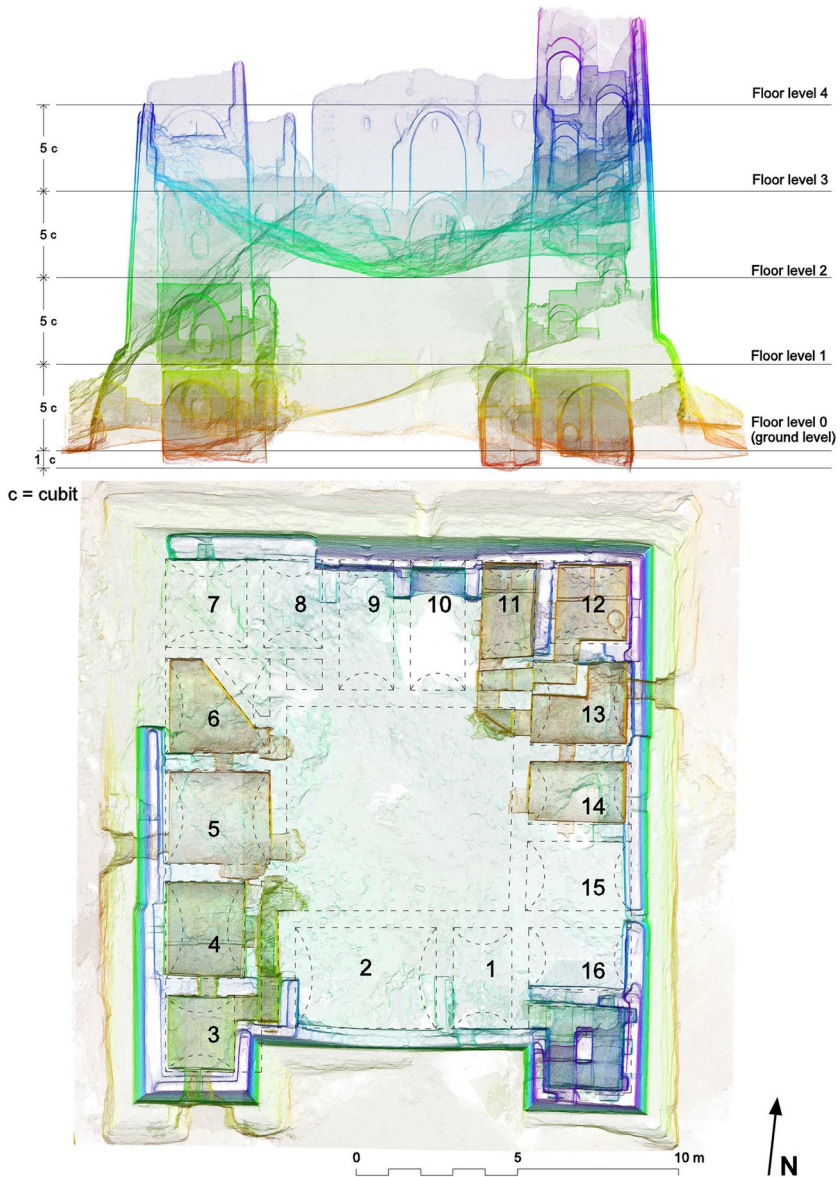
Fig. 7 Top and frontal view of the three-dimensional point model of the Fort and numbering system adopted to identify the rooms (height of the color range corresponding to 60 cm, drawing by F. Fiorillo)
