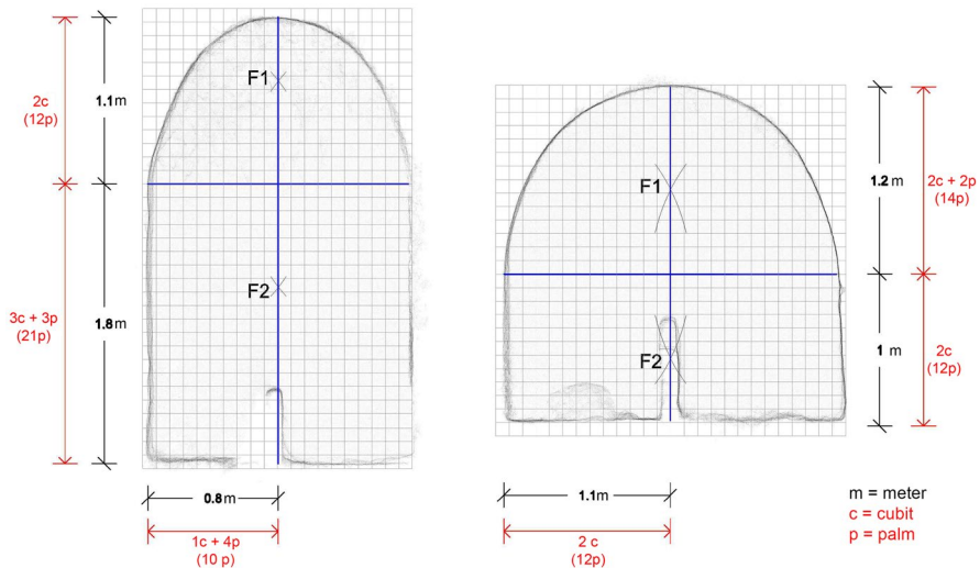
Fig. 11 1 palm square grid superimposed on the vertical section of rooms 0–13 and 0–14 highlighting the difference in palms between the rise and half of the clear span of the two arches (drawing by F. Fiorillo)
