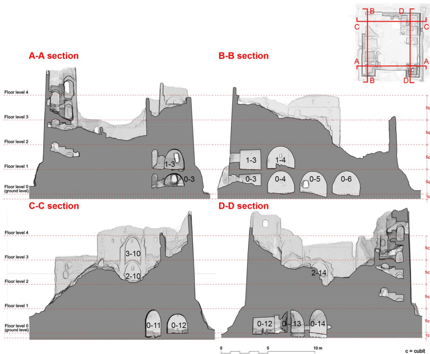
Fig. 8 Vertical sections of the Fort of Umm al-Dabadib, cut near the external walls: A-A, looking southwards; B-B, looking westwards; C-C, looking northwards; and D-D, looking eastwards (drawing by F. Fiorillo)
