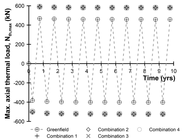
Fig. 4. Pile thermal axial load (tension positive).
