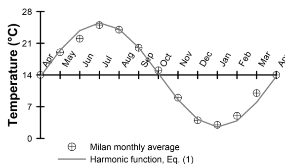
Fig. 2. Milan average monthly temperatures compared with Equation (1). Temperature data from - https://www.timeanddate.com/weather/italy/milan/climate
