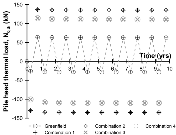
Fig. 5. Thermal reaction mobilised against pile cap.
