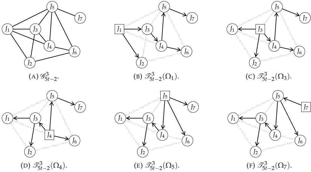
FIGURE 5.1. The spanning trees of \mathcal{G}_{5t-2}^3 determined using Theorem 5.4 and varying the hilb-segment ideal.
