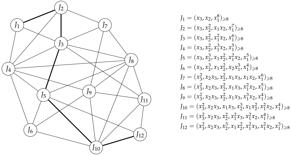
(A) The Borel graph \mathcal{G}_8^3 . The path connecting J_1 and J_{12} constructed in the proof of Proposition 5.11 is highlighted with a thick line.
