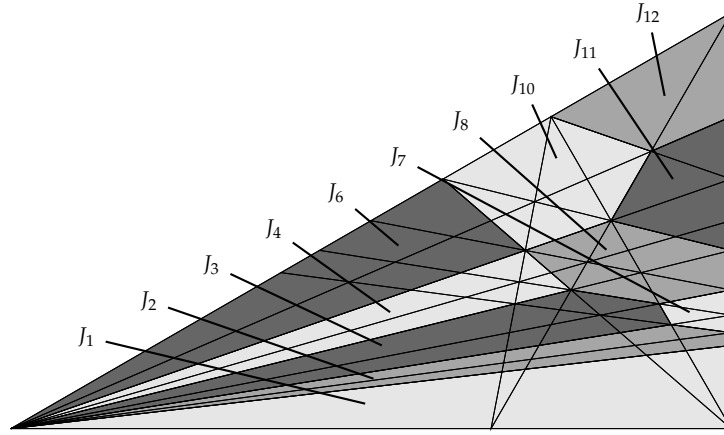
(B) The Gröbner fan \text{GF}(\mathbf{Hilb}_8^3) . Adjacent polygons colored with the same shade of gray corresponds to term orders \Omega whose degeneration graphs have the same maximum in \mathcal{S}_8^3 with respect to \succeq_{\Omega} .
