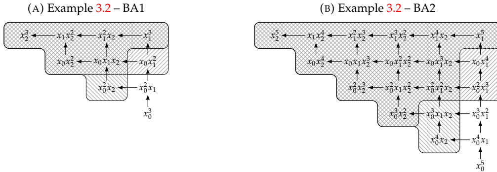
FIGURE 3.1. Examples of Borel adjacent pairs of strongly stable ideals in the polynomial ring \mathbb{K}[x_0, x_1, x_2] .
