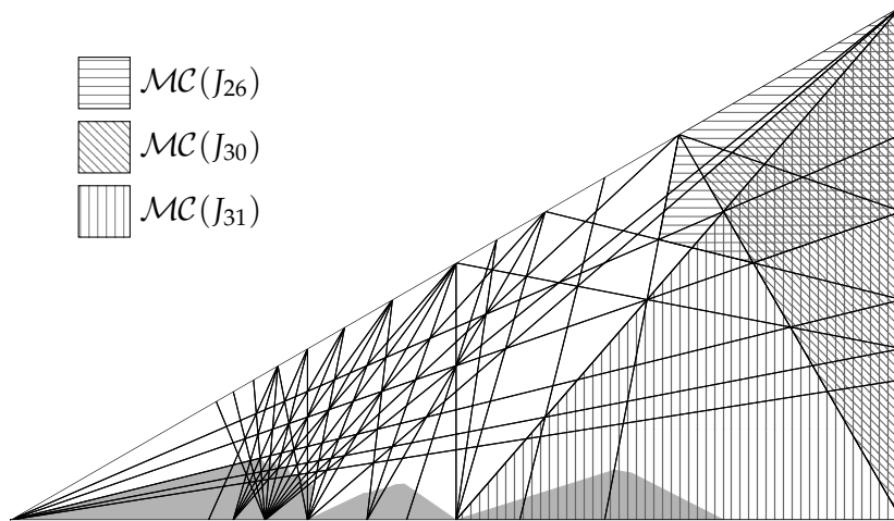
(B) The Gröbner fan \text{GF}(\mathbf{Hilb}_{6t-3}^3) . The maximality cones of J_{26} , J_{30} and J_{31} are highlighted with horizontal, oblique and vertical lines. The gray area corresponds to the union of all segment cones.
