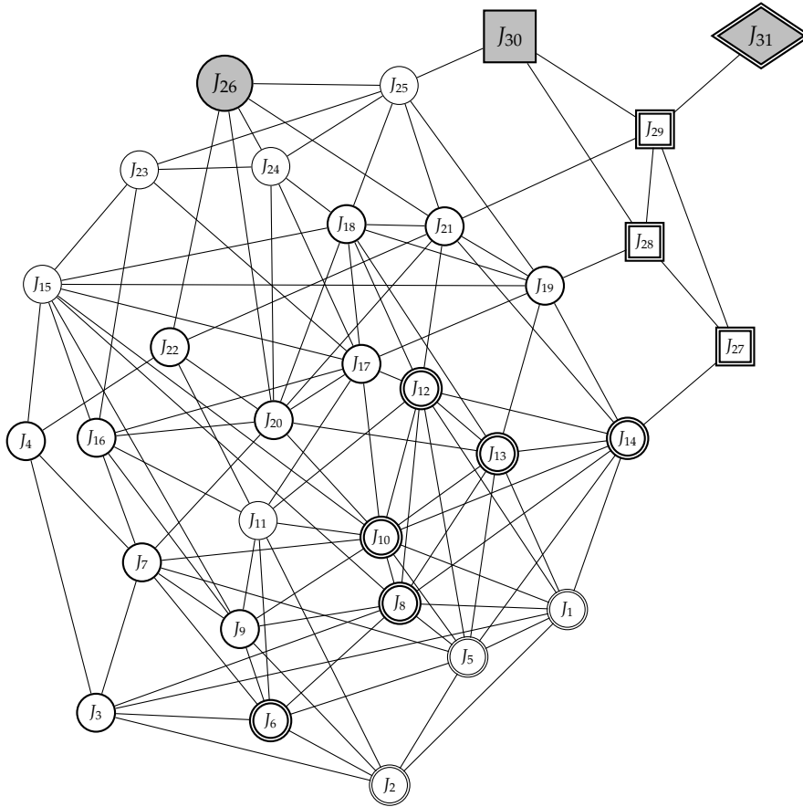
(A) The Borel graph \mathcal{G}_{6t-3}^3 . Regular ideals are drawn with a thin line, while irregular ideals are drawn with a thick line. Hilb-segment ideals are marked with a double line. Circle shaped vertices correspond to ideals with plane section (x_3, x_2^6) , squared shaped vertices correspond to ideals with plane section (x_3^2, x_2x_3, x_2^5) and the diamond shaped vertex correspond to the ideal with plane section (x_3^2, x_2^2x_3, x_2^4) . The gray bigger vertices are the maximal elements discussed in Example 5.21.
