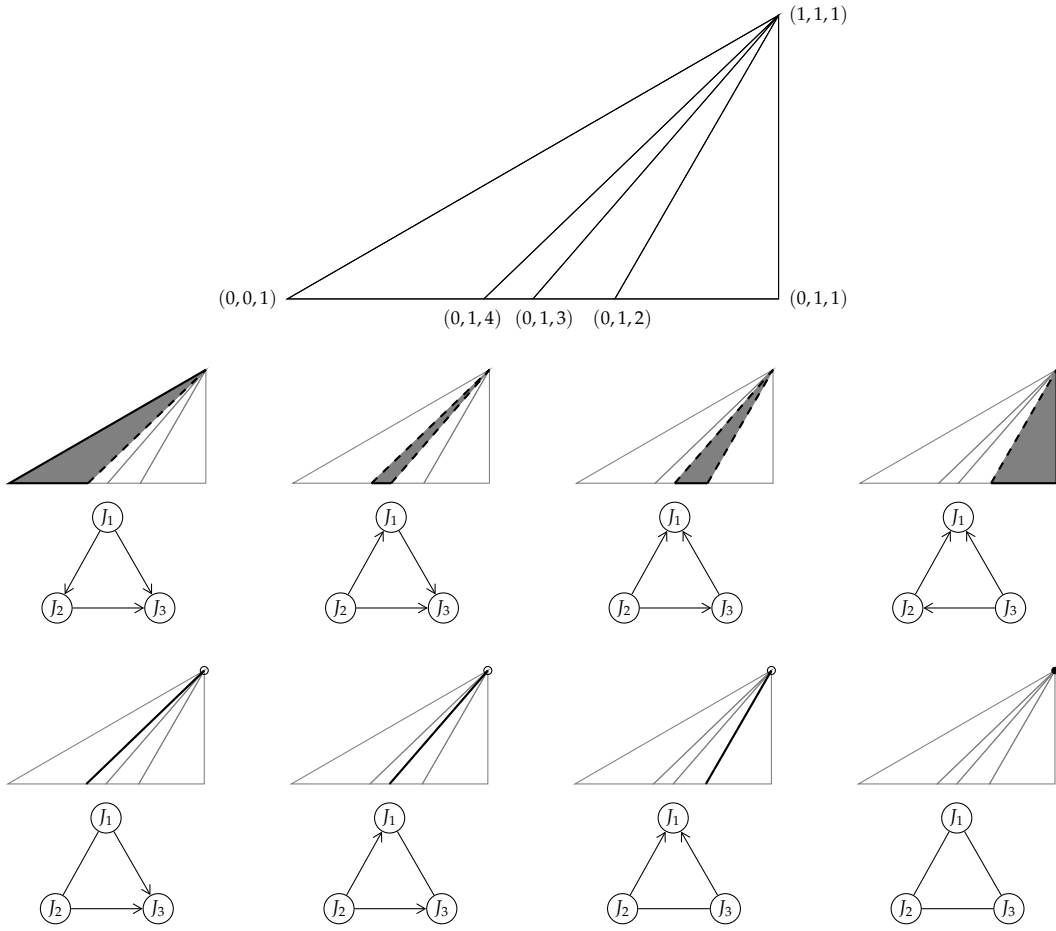
FIGURE 4.5. The Gröbner fan of the Hilbert scheme \mathbf{Hilb}_5^2 and the possible degeneration graphs.
