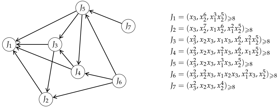
FIGURE 4.3. The RevLex-degeneration graph of the Hilbert scheme \mathbf{Hilb}_{5t-2}^3 .
