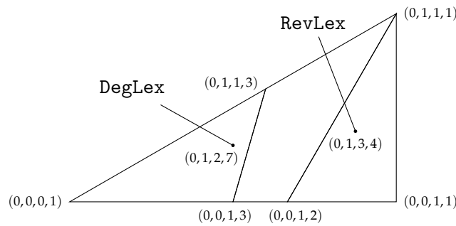
FIGURE 4.6. The Gröbner fan of the Hilbert scheme \text{Hilb}_{3t+1}^3 .
