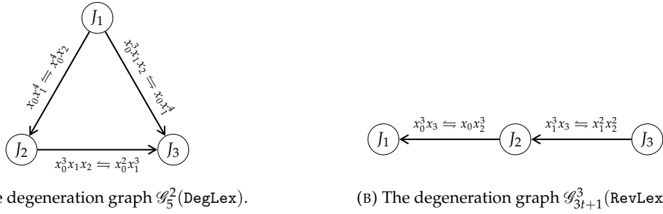
FIGURE 4.2. The degeneration graphs of \mathbf{Hilb}_5^2 with respect to the graded lexicographic order and of \mathbf{Hilb}_{3t+1}^3 with respect to the graded reverse lexicographic order.
