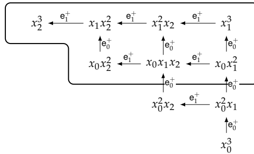
FIGURE 2.1. The Borel order \geq_B on the set of monomials \mathbb{T}_3^2 and the Borel set \mathfrak{J} corresponding to the ideal J^{\text{sat}} = (x_2^2, x_1 x_2, x_1^2) \subset \mathbb{K}[x_0, x_1, x_2] .
