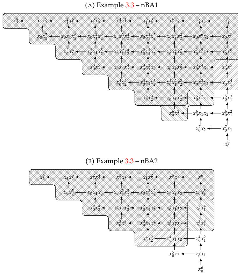
FIGURE 3.2. Examples of non Borel adjacent pairs of strongly stable ideals in the polynomial ring \mathbb{K}[x_0, x_1, x_2] .
