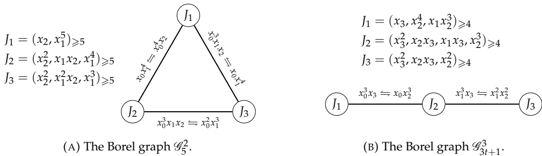
FIGURE 4.1. The Borel graph of the Hilbert schemes \mathbf{Hilb}_5^2 and \mathbf{Hilb}_{3t+1}^3 .
