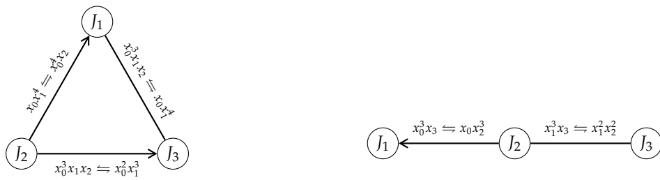
(A) The degeneration graph \mathcal{G}_5^2((0, 1, 3)) .
