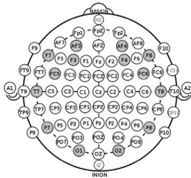
Figure 3. Emotiv Epoc+ electrodes highlighted in grey against the 10–10 I.S. layout and experiment setup using the headset.
