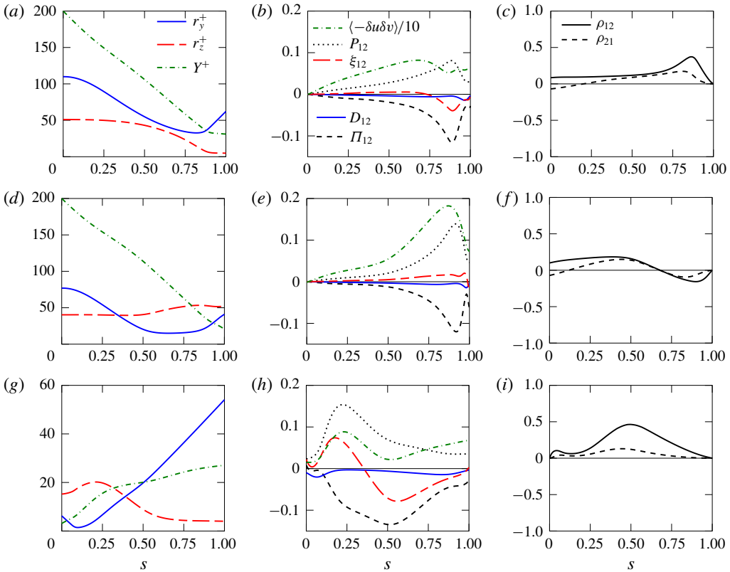
FIGURE 6. Field lines of the flux vector for \langle -\delta u \delta v \rangle . (a–c) Set I; (d–f) Set II; (g–i) Set IV. (a,d,g) Evolution of the values of Y (---, dark green), r_y (—, blue), r_z (—, red), along a representative field line as a function of its dimensionless arc length s . (b,e,h) Values of \langle -\delta u \delta v \rangle / 10 (---, dark green), \xi_{12} (—, red), P_{12} (·····), D_{12} (—, blue) and \Pi_{12} (---, grey) along the line. (c,f,i) Evolution of -\rho_{12} (—) and -\rho_{21} (---) along the line.
