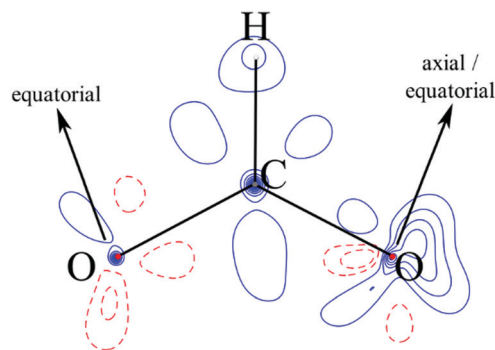
Fig. 5 Difference between charge density distributions of eq-ax formate ion and eq-eq formate ion, where blue and red contours ( 0.2 \text{ e } \text{Å}^{-3} ) represent, respectively, positive and negative regions of electron charge density.
