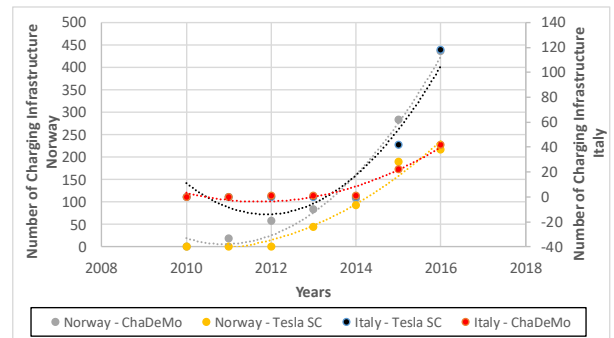
Fig. 6. Trend of the number of CHAdeMO and Tesla charging stations in Norway and Italy.
