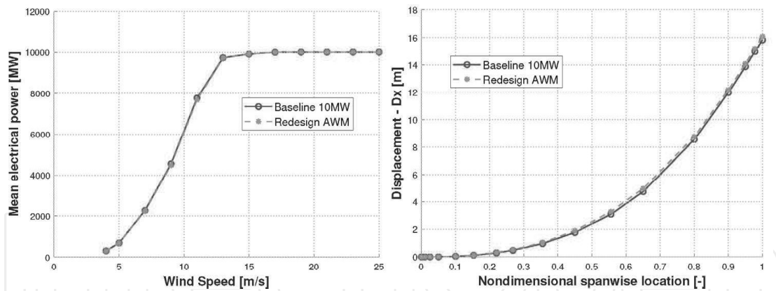
Figure 8. Power curves (left) and maximum blade deflections (right) for the baseline model and the optimized one.
