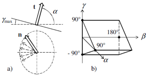
Fig. 3: Allowable combinations of variables: a) relation between \gamma and \alpha ; b) domain of the angles
