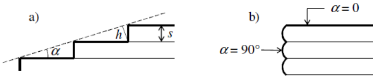
Fig. 4: Staircase effect: a) generic edge; b) horizontal and vertical edges
