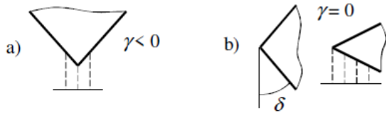
Fig. 5: Support effect: a) downward-pointing edges; b) laterally-pointing edges
