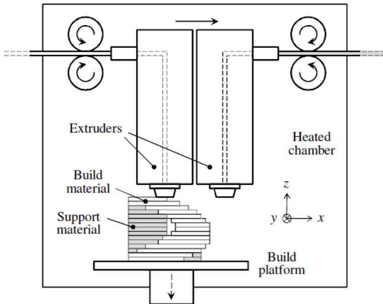
Fig. 1: Schematic of the FDM process
