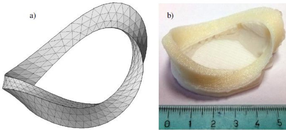
Fig. 10: Ring-shaped part: a) triangle mesh: b) FDM part with support
