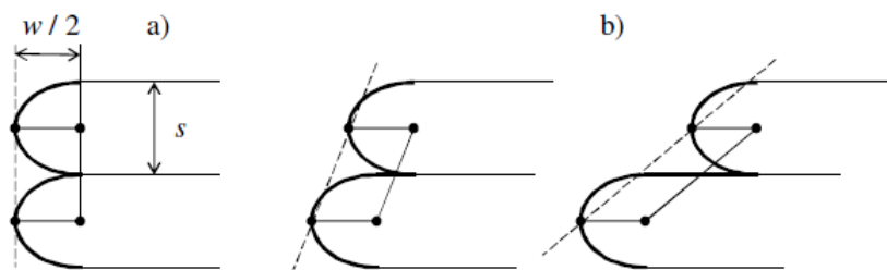
Fig. 7: Offset and curved-layer effect: a) vertical edges; b) inclined edges
