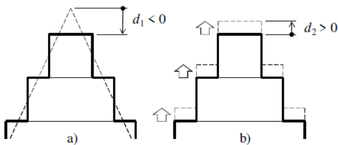
Fig. 8: Effects for \alpha = 0 : a) slicing error; b) swelling
