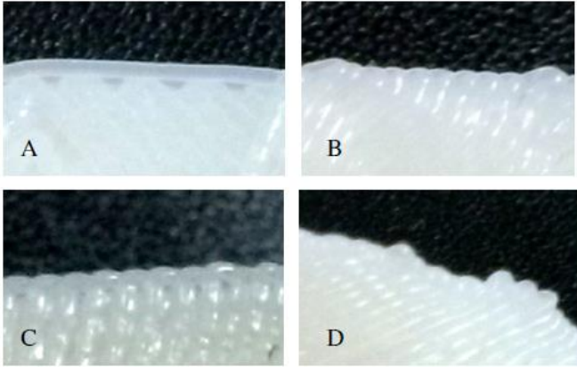
Fig. 12: Detail views on the ring-shaped part (refer to notes in Fig. 11)
