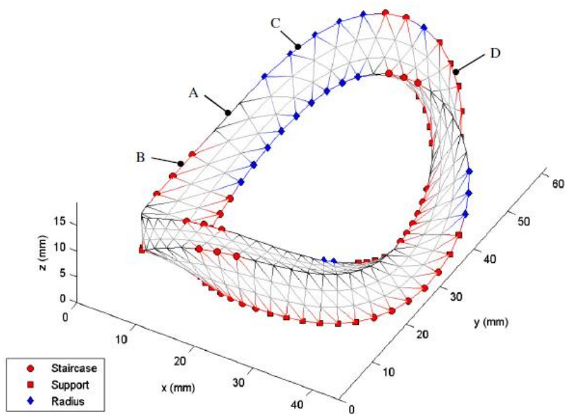
Fig. 11: Visualization of the process map on the ring-shaped part
