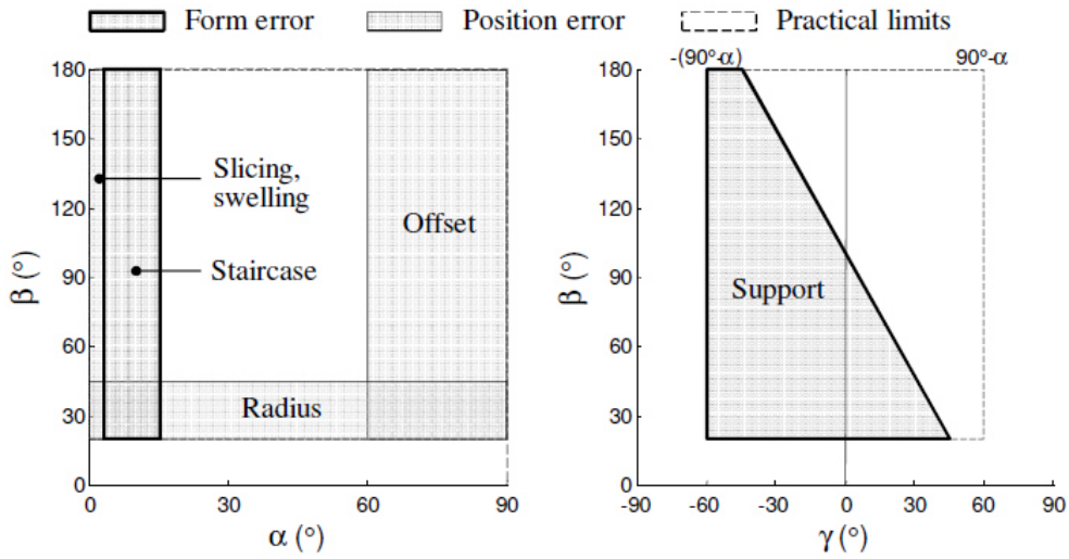
Fig. 9: Process map
