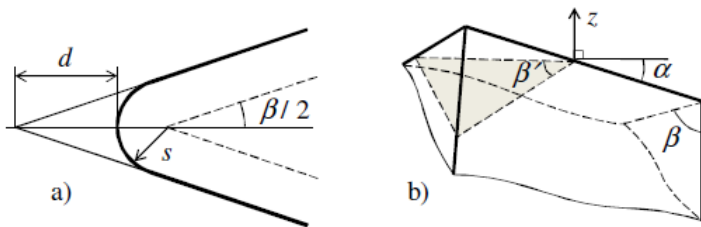
Fig. 6: Radius effect: a) deposition trajectory at an edge; b) bend angle
