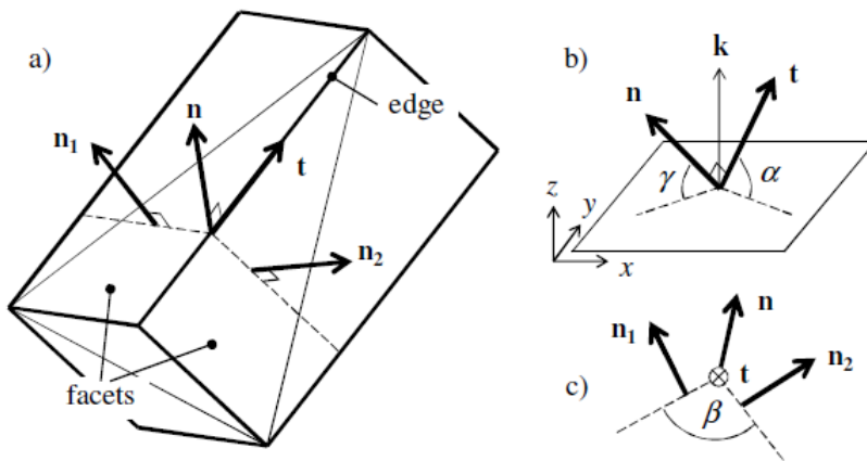
Fig. 2: Geometric entities associated to an edge: a) unit vectors; b) angles to the horizontal plane (inclination, incidence); c) angle defined on the normal plane (included)
