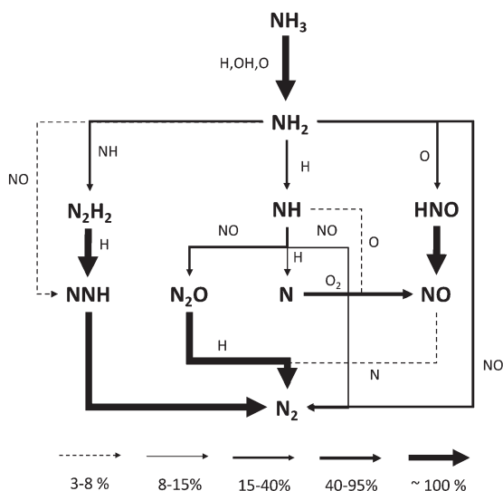
Fig. 12 Reaction flux analysis in FR at T = 1523 K and at a reactor length of 55 cm. Flux intensity is relative to the single molecule. For the sake of clarity, reactions between two N-molecules are reported only once.
