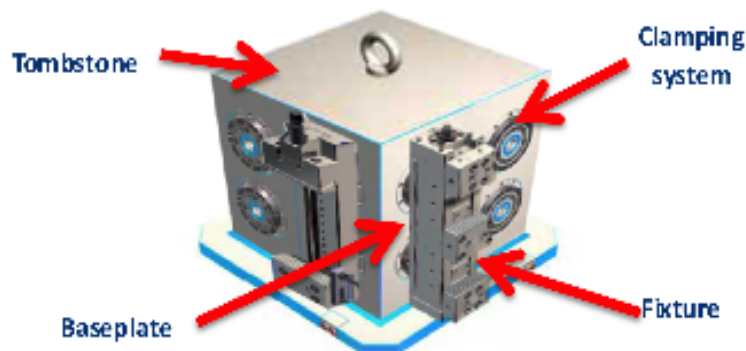
Fig. 1: Modular and reconfigurable pallet.
