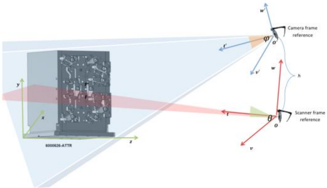
Fig. 4: Pallet scan process.
