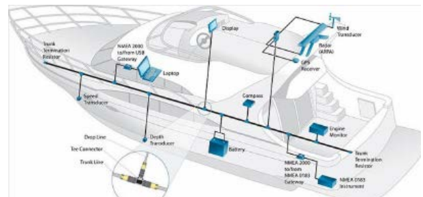
Figure 3: LINCOLN IoT Gateway
