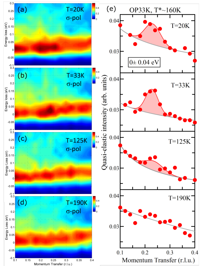
FIG. 5. (color online) Temperature dependence of charge order across T_c \simeq 33 K and T^* \simeq 160 K for OP33K. Energy/momentum intensity maps of RIXS spectra along (0,0) - (0.5,0) symmetry direction measured at (a) 20 K, (b) 33 K, (c) 125 K and (d) 190 K with \sigma polarization on OP33K. (e) Corresponding intensity at 0 \pm 0.04 eV for the quasi-elastic signal. Solid lines are Lorentzian fits to the data with a power law background. The areas after subtracting the background are highlighted by the red shading.
