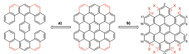
Figure 1. Possible pathways toward HBC with four additional K-regions (red).
