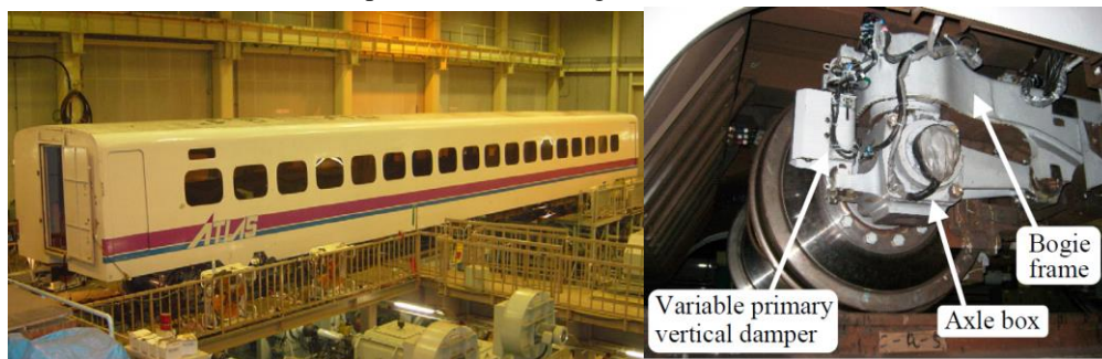
Figure 21 - Roller stock test plant [69] (Left) and installation of Semi-active primary vertical damper [41] (Right)
