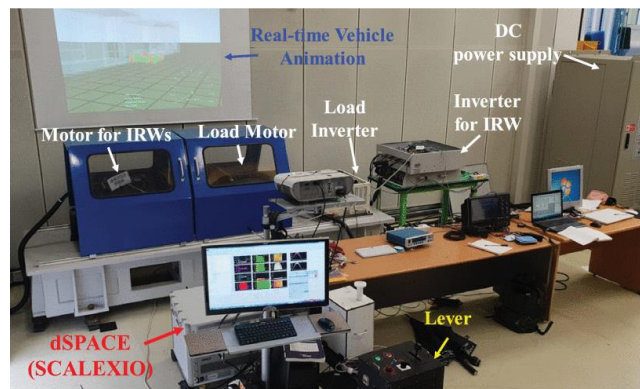
Figure 35 - Hardware in the loop test configuration [158]
