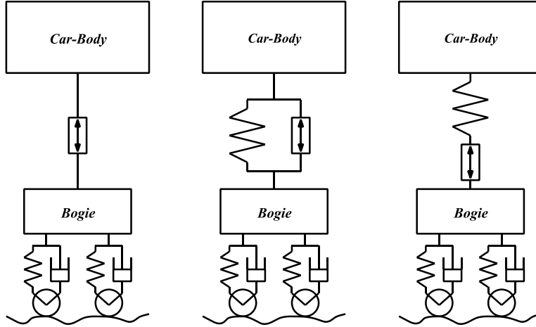
Figure 6 - Mechanical configurations of active secondary suspension
