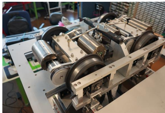
Figure 33 - 1:5 scaled test rig for high-depth subway system [140]
