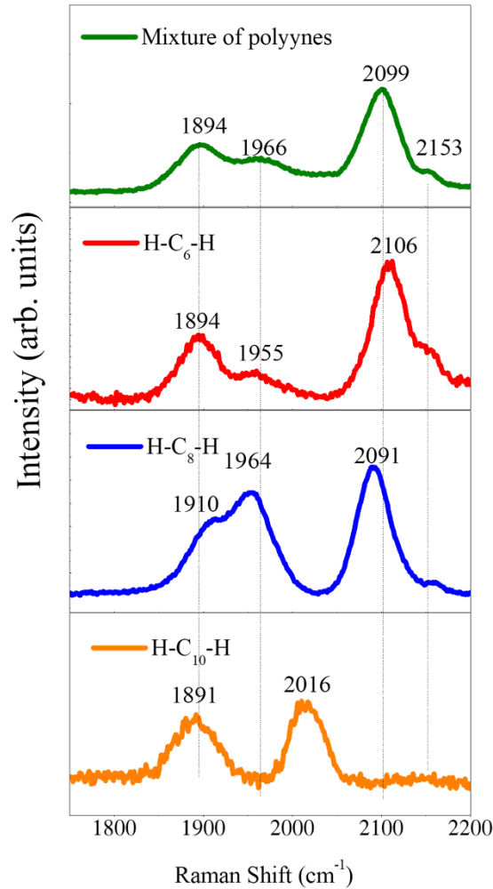
Figure 4. SERS spectra of a) the polyynes mixture, b) size-selected polyynes with n=6 , c) n=8 and d) n=10 .
