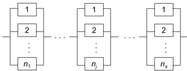
Figure 1: Series-Parallel System
