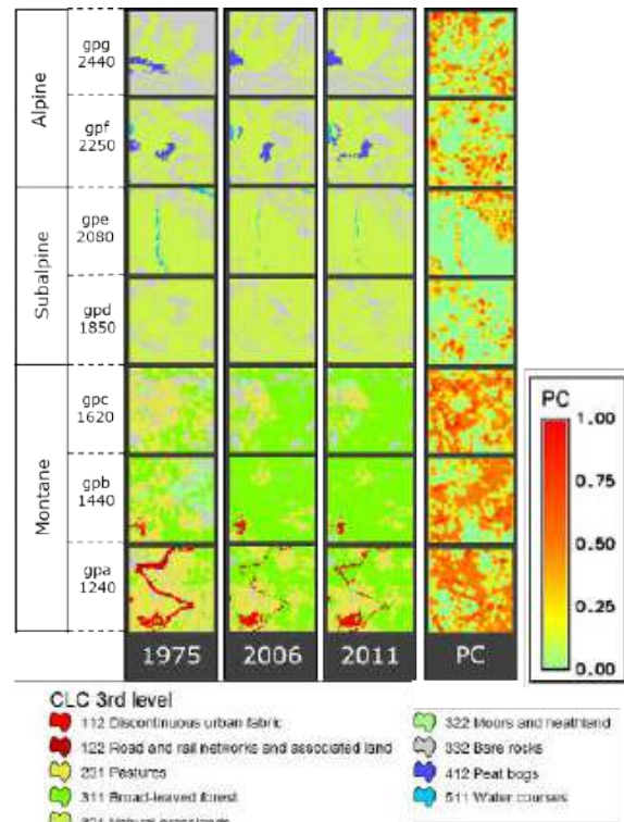
Figure 2. Results. 1975, 2006, 2011 classified and resampled products according to CLC legend. The elevation (m a.s.l.) and the altitudinal belt of each plot are listed. The proportion of change (PC) is a heat map where higher numbers correspond to major cell changes.
