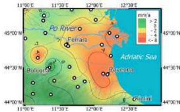
Figure 3 - Calibration map for PS vertical velocity to apply to PS to obtain "absolute" and corrected vertical velocity rates.
