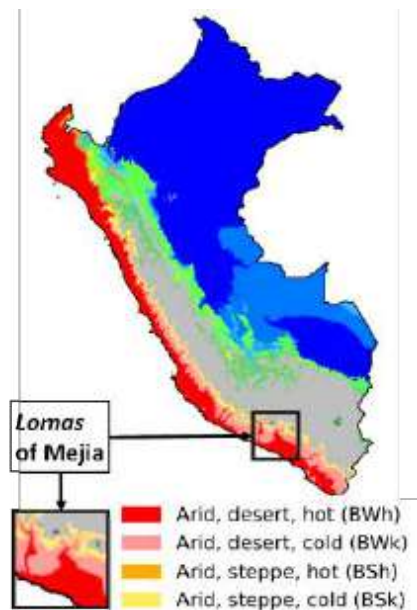
Figure 2. Location of the study area and climate zones of the Lomas de Mejia, processed from Beck et al., 2018.
