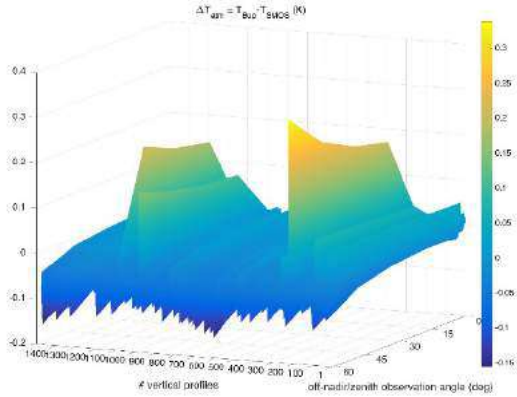
Figure 3. Atmospheric temperature difference between modeled self-emitted upward T_{Bu} and SMOS prediction T_{Bsm} .
