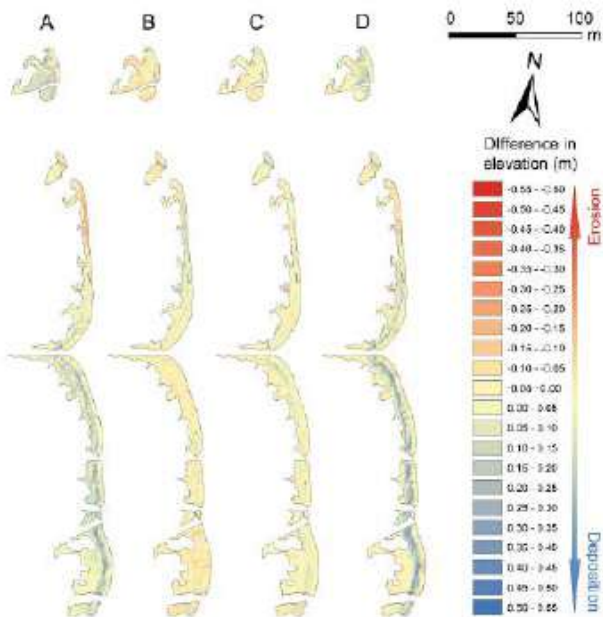
Figure 3 - Geomorphic variation of the incipient dune during the monitoring period: Dem of Difference (DoD) from March to Sep. 2017 (A); from Sep. to Dec. 2017 (B); from Dec. 2017 to Apr. 2018 (C) and cumulative period from March 2017 to Apr. 2018 (D).
