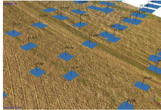
Figure 2. Dense Cloud Point of the study area (in blue the position of the photo in the space)
