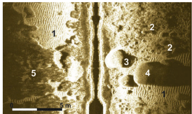
Figure 8 - Side Scan Sonar image (1MHz – 8 meter depth) – Sella del Diavolo cliff. 1) Megaripples structures on Silicoclastic sediments ( \lambda= 0.5\div 1 m); 2) elaborated landslide deposits; 3) Block fall (d=4 m h= 3m); 4) Block fall (d=6 m h= 5m); 5) Posidonia oceanica on wave-cut platform.
