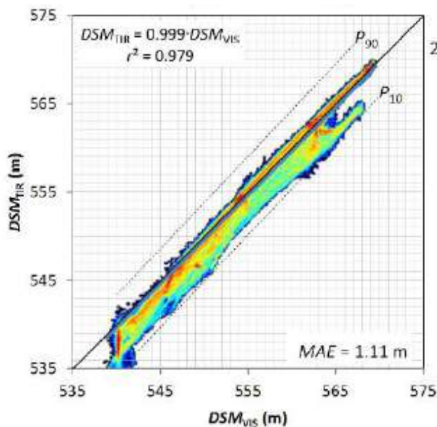
Figure 12. DSM_{VIS} from an overpass under direct plus diffuse solar radiation versus DSM_{TIR} from an overpass just after sunrise under diffuse solar radiation.
