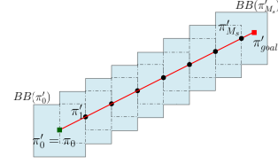
Fig. 2. Procedure to compute the minimum number of bounding boxes: tile the straight line between \pi_0 \pi'_goal using the projection of the bounding box on the position space (here shown as \mathbb{R}^2 ).
