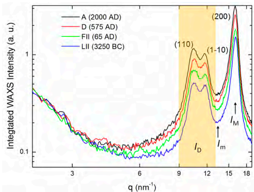
Figure 3. One-dimensional WAXS profiles extracted from the relevant 2D patterns after integration in the angular sector of 10 degrees around the hk0 equatorial fiber-diffraction axis in arbitrary units: The cellulose (110) and (1–10) diffraction peaks have been indexed and rescaled to have the same integrated intensity in the q -range 1.5\text{--}4.0\text{ nm}^{-1} . See the main text for further details and Table 1 for symbols.
