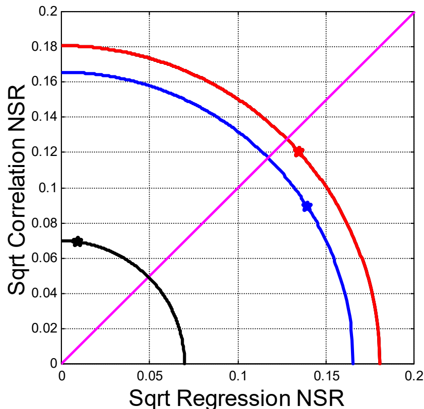
Figure A2. From X-ray to ^{14}\text{C} measurements: Square root of the noise-to-signal ratio ( \text{NSR} ) as a function of the square root of the regression \text{NSR}_a (abscissa) taken as the absolute value |a - 1| and the square root of the correlation \text{NSR}_r (ordinate): The black line is the central values of column 3 in Table 3. The blue line is +2\sigma . The red line is -2\sigma . The 45^\circ line shows where \text{NSR}_r = \text{NSR}_a .
