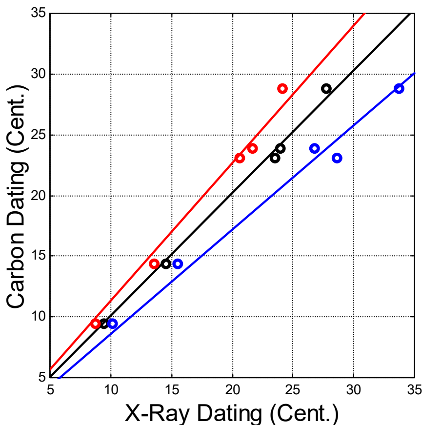
Figure A1. Scatter plots and their best-fit regression lines between (i) the central values of x vs. y (black); (ii) the +2\sigma values of x vs. y (blue); and (iii) the -2 of x vs. y (red).
