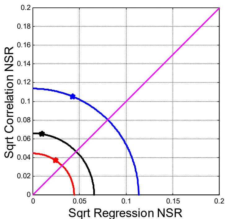
Figure A4. From ^{14}\text{C} to X-ray measurements: Square root of the noise-to-signal ratio (NSR) as a function of the square root of the regression \text{NSR}_q (abscissa) taken as the absolute value |a - 1| and the square root of the correlation \text{NSR}_r (ordinate): The black line is the central values of column 2 in Table 3. The blue line is +2\sigma . The red line is -2\sigma . The 45^\circ line shows where \text{NSR}_r = \text{NSR}_q .
