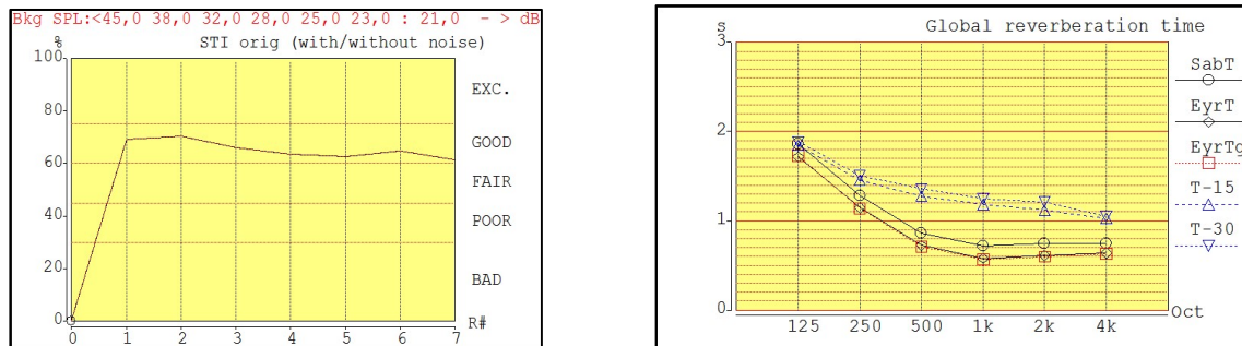
Figure 7 and 8: STI Values and Trend and RT Sabine (SabT), RT Eyring (EyrT), T_{30} and T_{15}
