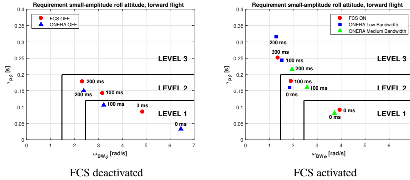
Fig. 13: Bandwidth and Phase Delay Comparison with [26].
