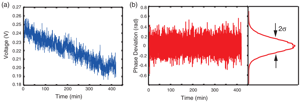
FIG. 3. Characterization of the AIS. (a) Evolution of the control voltage applied to the piezo translation stage while operating the AIS over 7 h. (b) Variation of the recorded phase over the same time interval yielding a standard deviation of about 60 as.
