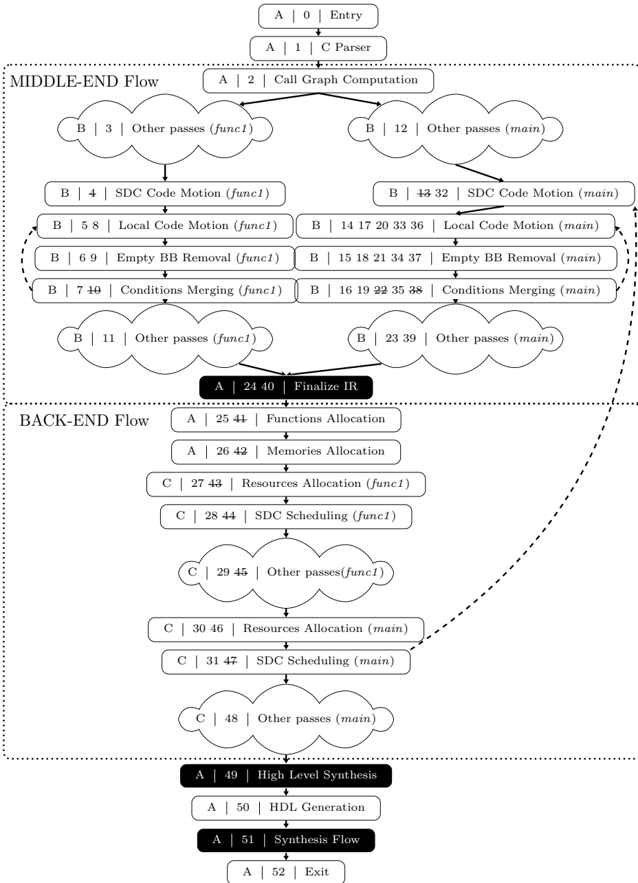
Fig. 1. Example of Design Flow Graph implementing the High Level Synthesis of a specification composed of two functions ( func1 and main ). Black boxes are Composing passes . The letters identify the order of insertion of the passes, the numbers identify the order of execution of the passes, the canceled numbers represent skipped passes while the dashed edges represent the invalidations. A passes are added at the beginning, B passes after iteration 2, C passes after iteration 26. For the sake of readability, a transitive reduction was applied.
