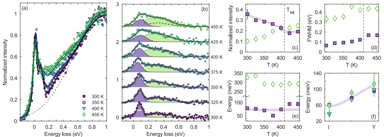
FIG. 2. Color online. Analysis of RIXS spectra collected at \Gamma - Y . (a): Representative low-energy RIXS spectra, each of which is normalized to the d-d excitations at 1 eV energy loss (dashed line). (b): Spectra with elastic line and d-d contributions subtracted off. Added are the best fit to the data (black solid line), and relative components of the magnon peak (purple) and high-energy continuum (green). Dashed line superimposed on 450 K plot is best fit to 300 K data for comparison. Yellow bar indicates FWHM of resolution function. (c–e): Fitted peak intensity (c), intrinsic FWHM (d), and energy (e) of the magnon peak (filled squares) and high-energy continuum (open diamonds) as a function of temperature. Solid lines are guides to the eye. (f): Energy of magnon peak as function of momentum transfer and temperature. The symbols are the same as part (a). Solid line is best fit to dispersion at 300 K as determined within Ref. 26.
