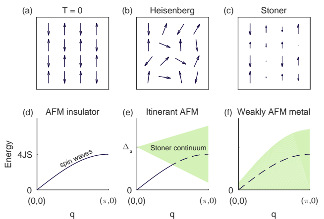
FIG. 1. Color online. Top panels: Schematic of the orientation of antiferromagnetically (AFM) interacting magnetic moments on a square lattice for T = 0 , and finite temperatures in the Heisenberg or Stoner limits. Bottom panels: Excitation spectra in the Heisenberg limit, for an itinerant AFM (with critical energy scale \Delta_s ), and for a metal with weak AFM correlations. Dashed lines indicate damped excitations.
