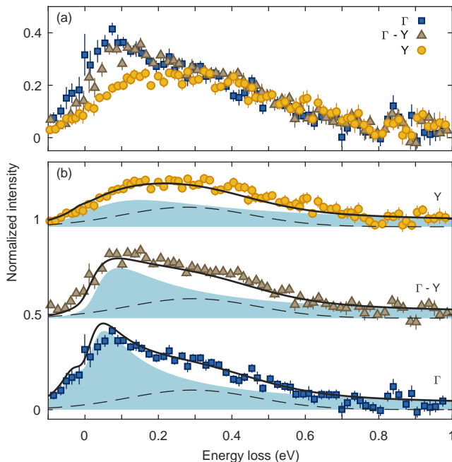
FIG. 3. Color online. Paramagnetic spin fluctuations (SF) in NaOsO 3 at 450 K. (a): Experimental data collected at various crystal momenta. For clarity the elastic line and high-energy intra- t_{2g} excitations have been subtracted. (b): Comparison of WAFL model (solid line) with experimental data. Filled area indicates paramagnetic SF calculated using Equation 1, with \gamma = 0.02 \text{ meV}^{-1} and \xi/a_0 \sim 1 . Dashed line is a momentum-independent high-energy contribution, which likely results from inter-band particle-hole excitations.
