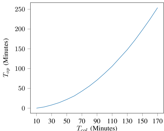
Fig. 9. Time needed to perform the operations on the shares vs Period of collection of the shares (an arrival rate \lambda = 1req/s is considered)
