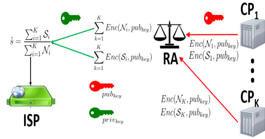
Fig. 3. Secure computation of the average contents' size
