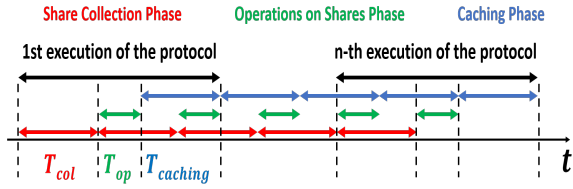
Fig. 2. Phases of the execution of the NN-compliant protocol
