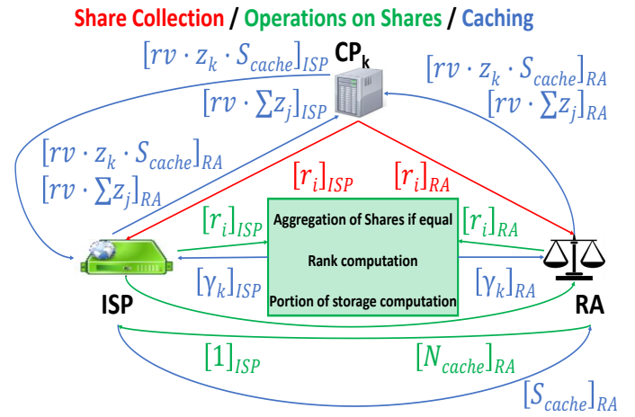
Fig. 4. Main shares learnt by ISP, CPs and RA during the execution of the NN-compliant protocol
