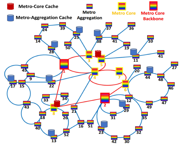
Fig. 5. Schematic representation of the ISP Network Topology and the location of caches.
