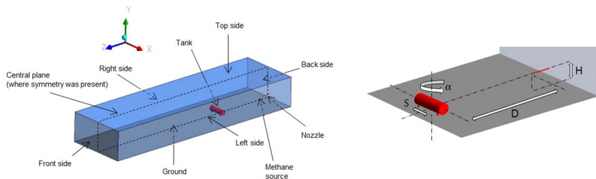
Figure 1: a) Computational domain represented as a full 3D; b) Geometric key parameters
