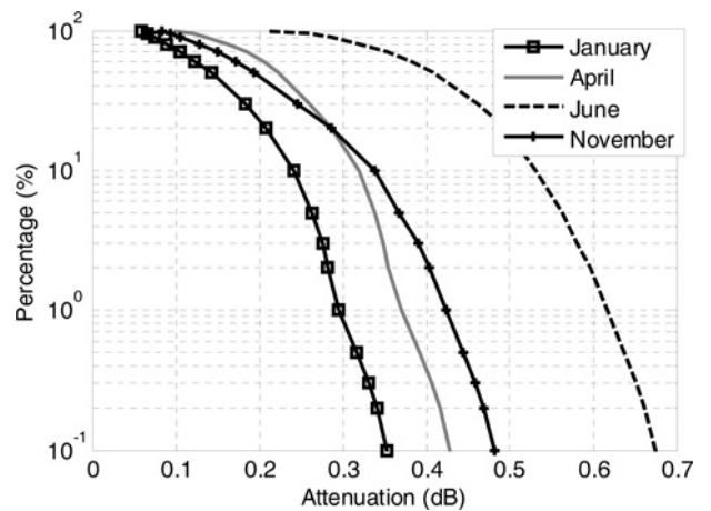
Fig. 4 Example of the monthly P(A_v) due to water vapour predicted by ITU-R recommendation P. 676-10 for the months reported in Fig. 1, using the characteristics of the radio link established between the Spino d'Adda station and the ITALSAT satellite (elevation angle of 37.7°, 39.6 GHz operation frequency)
