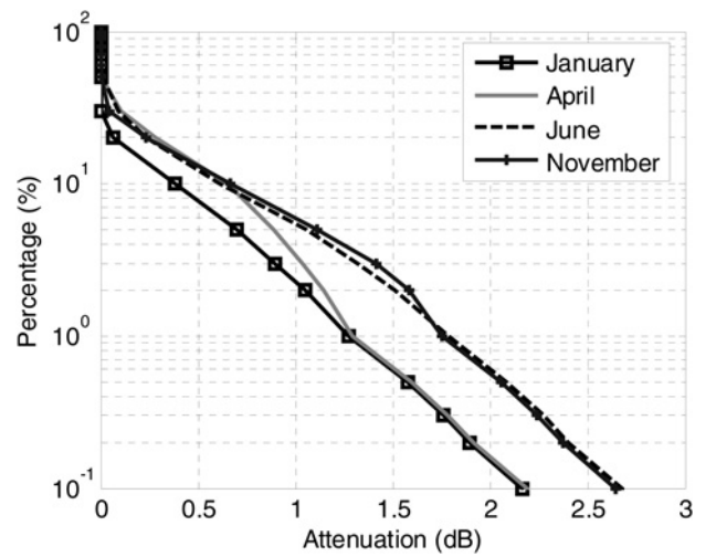
Fig. 3. Example of the monthly P(A_c) due to clouds predicted by ITU-R recommendation P. 840-6 for the months reported in Fig. 1, using the characteristics of the radio link established between the Spino d'Adda station and the ITALSAT satellite (elevation angle of 37.7°, 39.6 GHz operation frequency)
