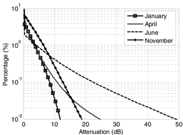
Fig. 2 Example of the P(A_R)^m 's predicted by SC EXCELL for the months reported in Fig. 1, using the characteristics of the radio link established between the Spino d'Adda station and the ITALSAT satellite (elevation angle of 37.7°, 39.6 GHz operation frequency and circular wave polarisation)
