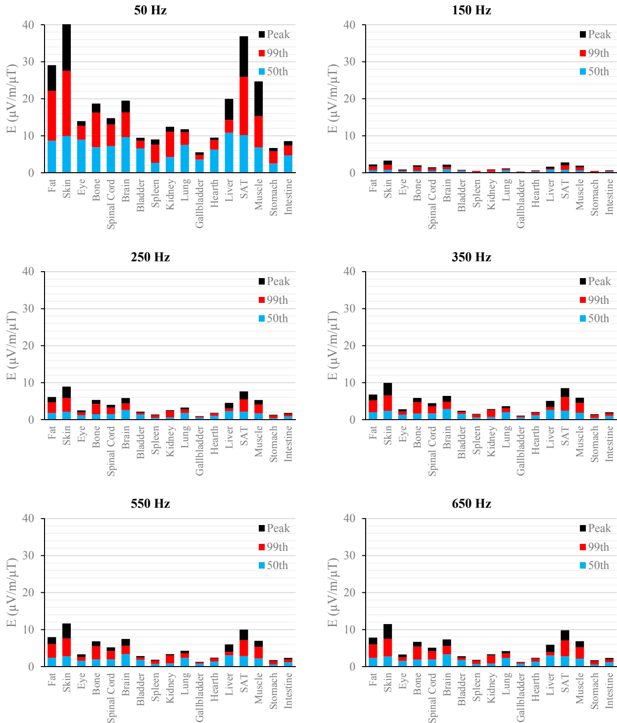
Figure 5. E ( \mu\text{V}/\text{m} ) per \mu\text{T} of 50 Hz B_{\text{peak}} induced in foetal tissues at 7 mGA for all the harmonic frequencies considering the standard EN 50160 for the HV power supply networks. The bars indicate the E_{50\text{th}} (blue), the E_{99\text{th}} (red) percentiles and the E_{\text{peak}} (black) of each distribution.
