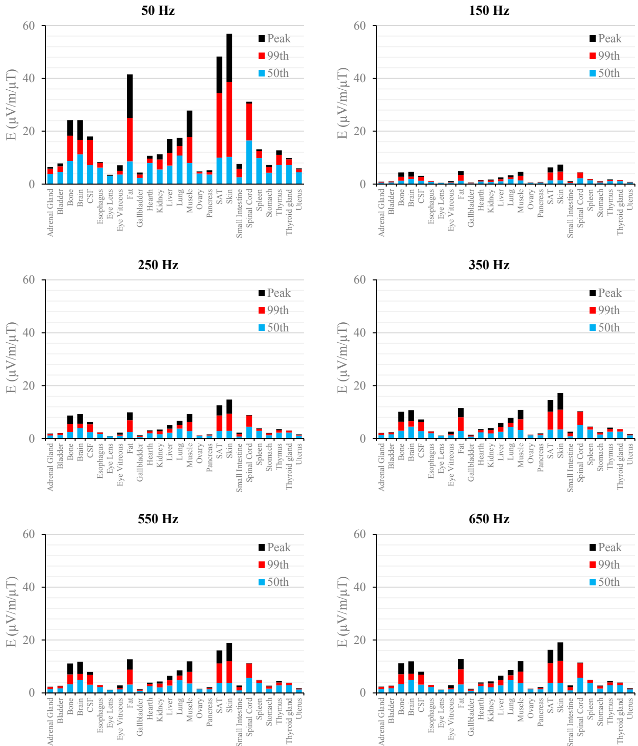
Figure 6. E ( \mu\text{V}/\text{m} ) per \mu\text{T} of 50 Hz B_{\text{peak}} induced in foetal tissues at 9 mGA for all the harmonic frequencies considering the standard EN 50160 for the LV&MV power supply networks. The bars indicate the E_{50\text{th}} (blue), the E_{99\text{th}} (red) percentiles and the E_{\text{peak}} (black) of each distribution.
