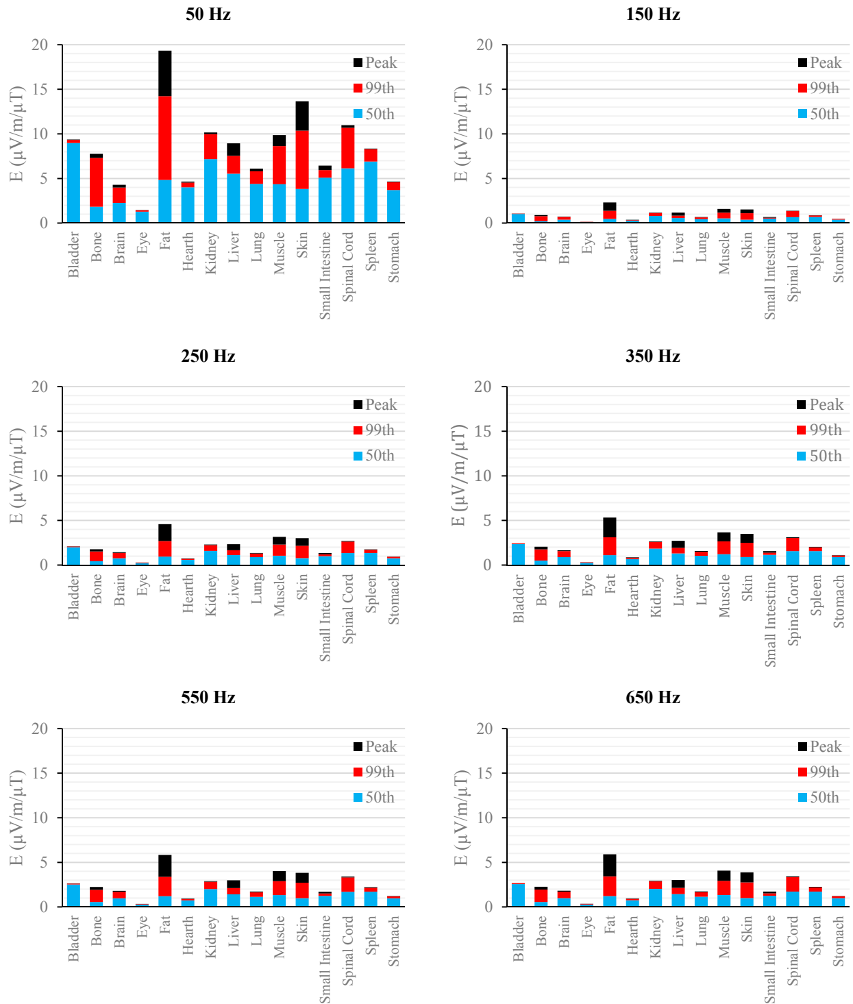
Figure 2. E ( \mu\text{V/m} ) per \mu\text{T} of 50 Hz B_{\text{peak}} induced in foetal tissues at 3 mGA for all the harmonic frequencies considering the standard EN 50160 for the LV&MV power supply networks. The bars indicate the E_{50\text{th}} (blue), the E_{99\text{th}} (red) percentiles and the E_{\text{peak}} (black) of each distribution.
