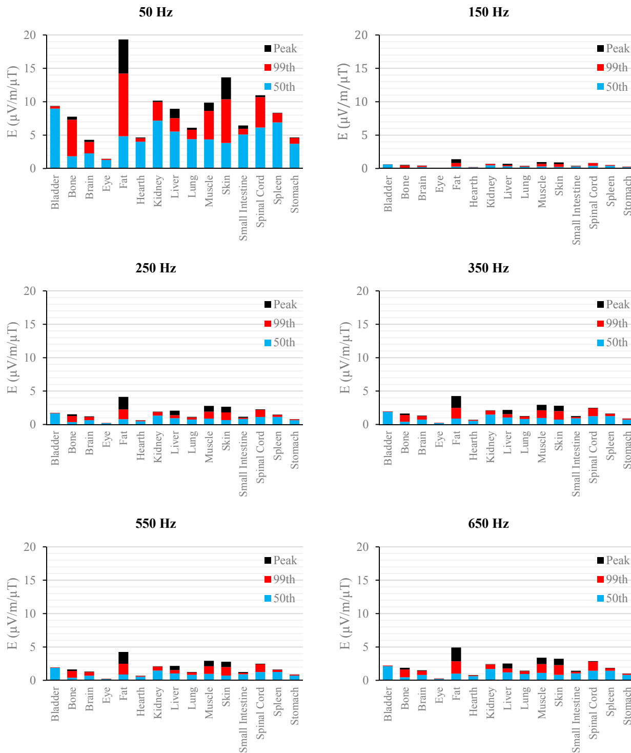
Figure 3. E ( \mu\text{V/m} ) per \mu\text{T} of 50 Hz B_{peak} induced in foetal tissues at 3 mGA for all the harmonic frequencies considering the standard EN 50160 for the HV power supply networks. The bars indicate the E_{50th} (blue), the E_{99th} (red) percentiles and the E_{peak} (black) of each distribution.
