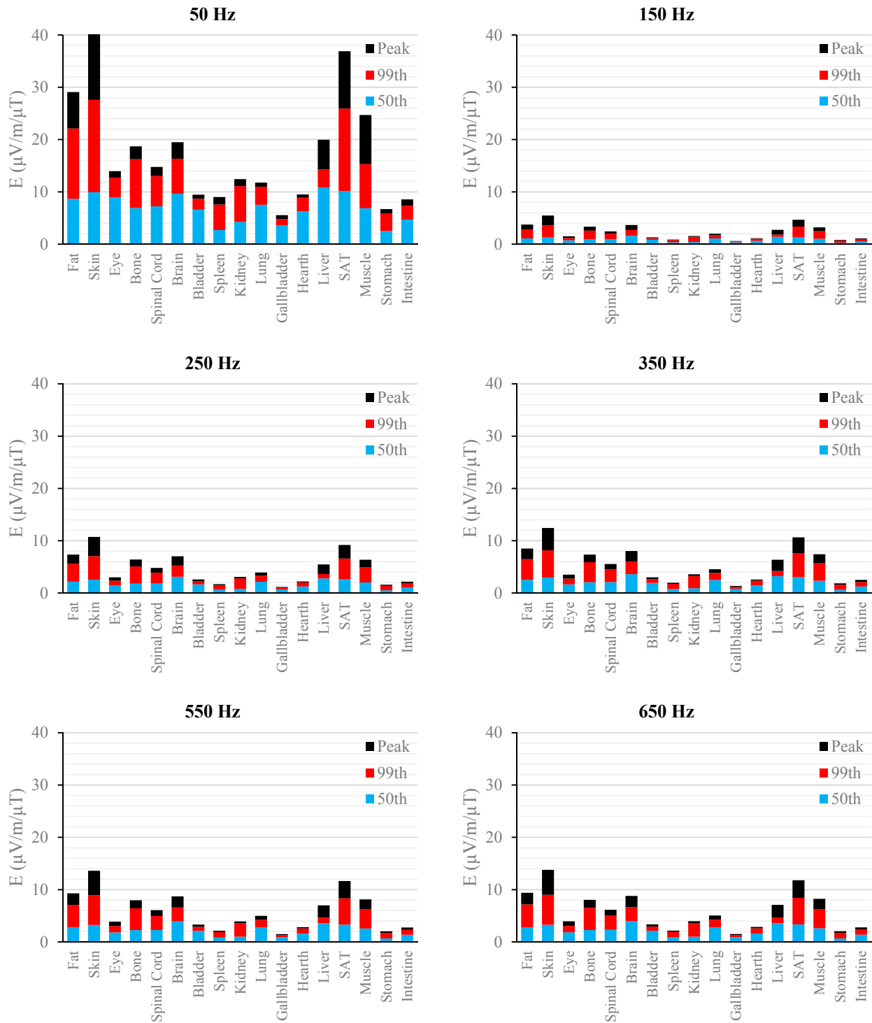
Figure 4. E ( \mu\text{V}/\text{m} ) per \mu\text{T} of 50 Hz B_{\text{peak}} induced in foetal tissues at 7 mGA for all the harmonic frequencies considering the standard EN 50160 for the LV&MV power supply networks. The bars indicate the E_{50\text{th}} (blue), the E_{99\text{th}} (red) percentiles and the E_{\text{peak}} (black) of each distribution.
