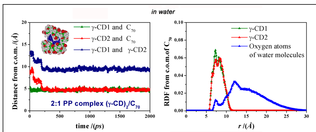
Figure 6. At left, the distance calculated during MD run in water between the c.o.m. of C_{70} and of the first \gamma -CD (the lower CD in the inset) in green, between the c.o.m. of C_{70} and of the second \gamma -CD (the upper CD) in red, and the distance between the c.o.m. of the two \gamma -CDs in blue for the PP complex. At right, the radial distribution function RDF calculated as a function of the distance r from the fullerene c.o.m. of the atoms of two different \gamma -CDs of the PP [(\gamma\text{-CD})_2/C_{70}] complex and of oxygen atoms of the water molecules.
