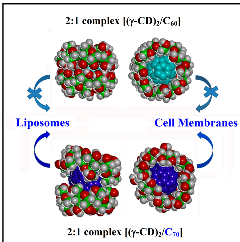
Figure 8. A sketch of the [( \gamma -CD) 2 /C 70 ] complex structure as obtained in the present theoretical work and of the analogous [( \gamma -CD) 2 /C 60 ] complex from [4] summarizing also the unlike experimental behavior [3]: the former complex exposes part of the hydrophobic fullerene surface than the latter one, and accordingly it is more prone to release the C 70 fullerene when in contact with the liposomes or cell membranes, as also shown in the sketch of Figure 1 based on experimental data [3].
