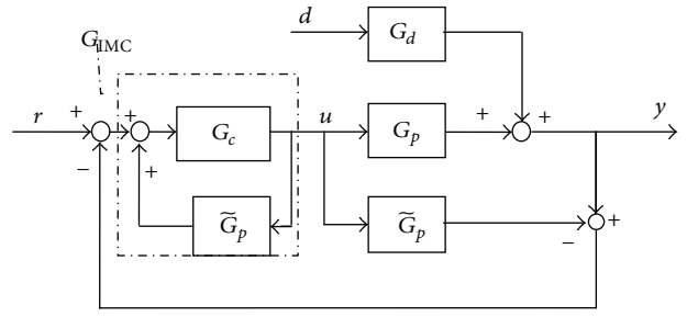
FIGURE 5: Relationship between the IMC structure and the feedback control structure.
