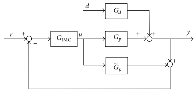
FIGURE 3: The IMC structure diagram.
