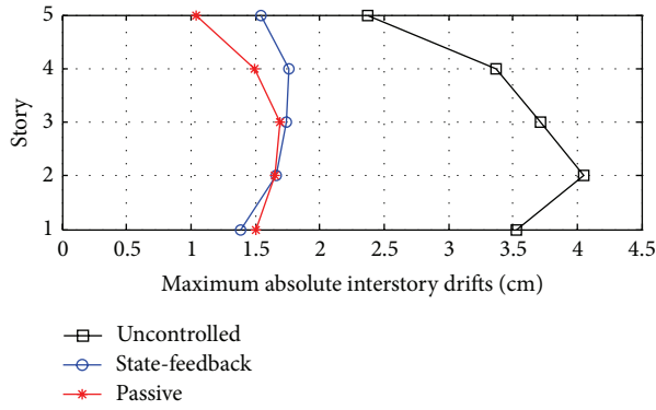
FIGURE 5: Maximum absolute interstory drifts corresponding to the uncontrolled building (black line with rectangles), the ideal state-feedback energy-to-peak controller defined by the gain matrix \bar{G}_s (blue line with circles), and the passive-damping system defined by the gain matrix \bar{K}_d (red line with asterisks). The full scale North-South El Centro 1940 seismic record has been used as ground acceleration disturbance.
