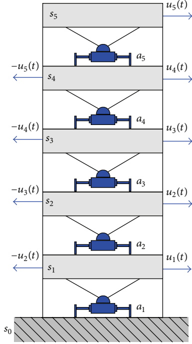
FIGURE 1: Five-story building actuation scheme.
