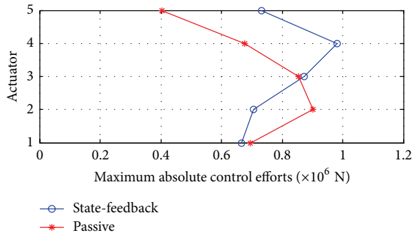
FIGURE 6: Maximum absolute control efforts corresponding to the ideal state-feedback energy-to-peak controller defined by the gain matrix \bar{G}_s (blue line with circles) and the passive-damping system defined by the gain matrix \bar{K}_d (red line with asterisks). The full scale North-South El Centro 1940 seismic record has been used as ground acceleration disturbance.
