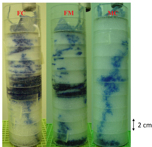
Figure 2. Three samples at the end of the experiments: FC2 (on the left, as an example of FC samples), FM2 (at the center, as an example of FM samples), and MC1 (on the right, as an example of MC samples).
