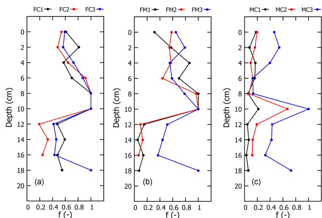
Figure 3. Measured f profiles. f is the ratio between wet and total area for all the sections in Fig. 1. (a) FC samples; (b) FM samples; (c) MC samples. The vertical coordinate refers to the depth of the section from sample top surface. Serial numbering 1–3 represent the three different input rates.
