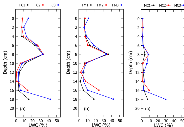
Figure 4. Measured LWC (vol %). (a) FC samples; (b) FM samples; (c) MC samples. Each point represents bulk LWC in the underlying 2 cm. This convention is consistent with Figs. 1 and 3. Serial numbering 1–3 represent the three different input rates.
