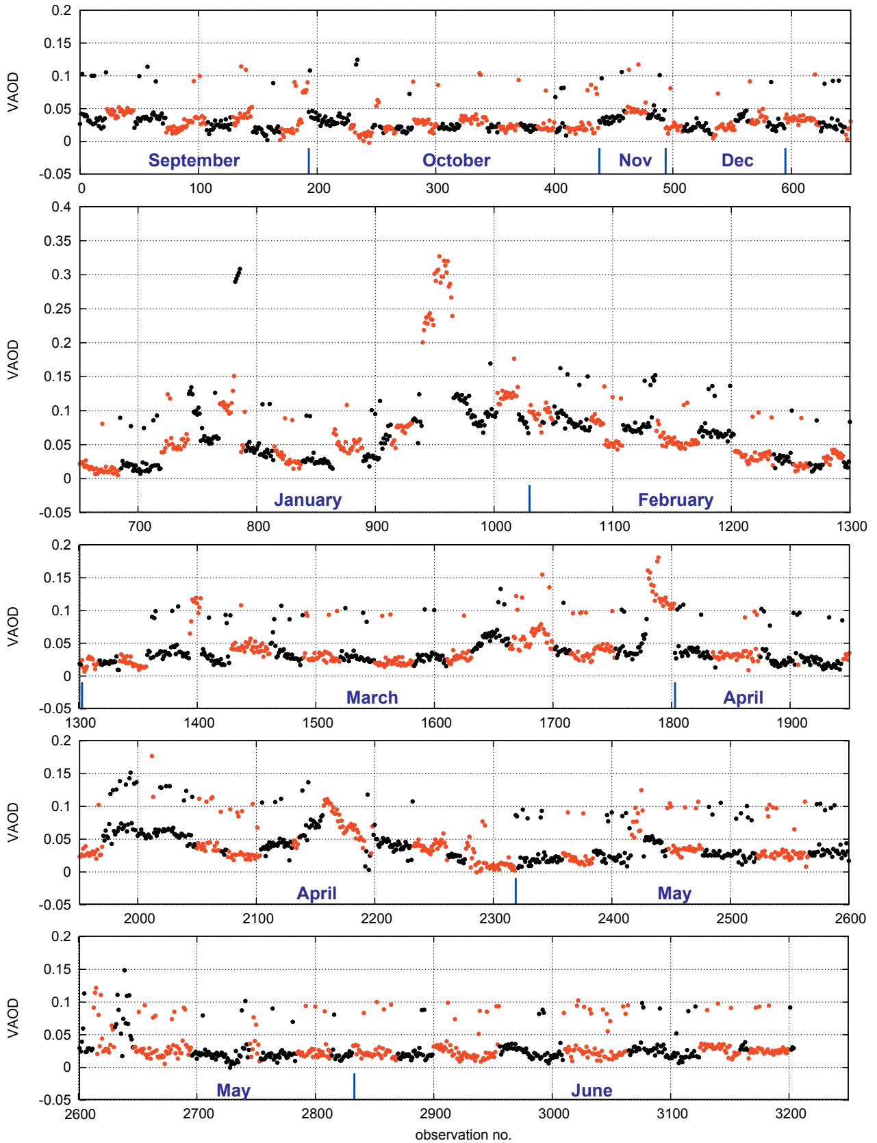
Figure 1. Time series of VAOD measurements taken by the CTA FRAM telescope located near Cerro Paranal in Chile from 09/2017 to 06/2018. Each point represents one scan in altitude from the zenith to the horizon in seven 30s exposures. Consecutive points of the same color were taken during the same night, but there can be several nights skipped due to weather or hardware issues for each color change.
