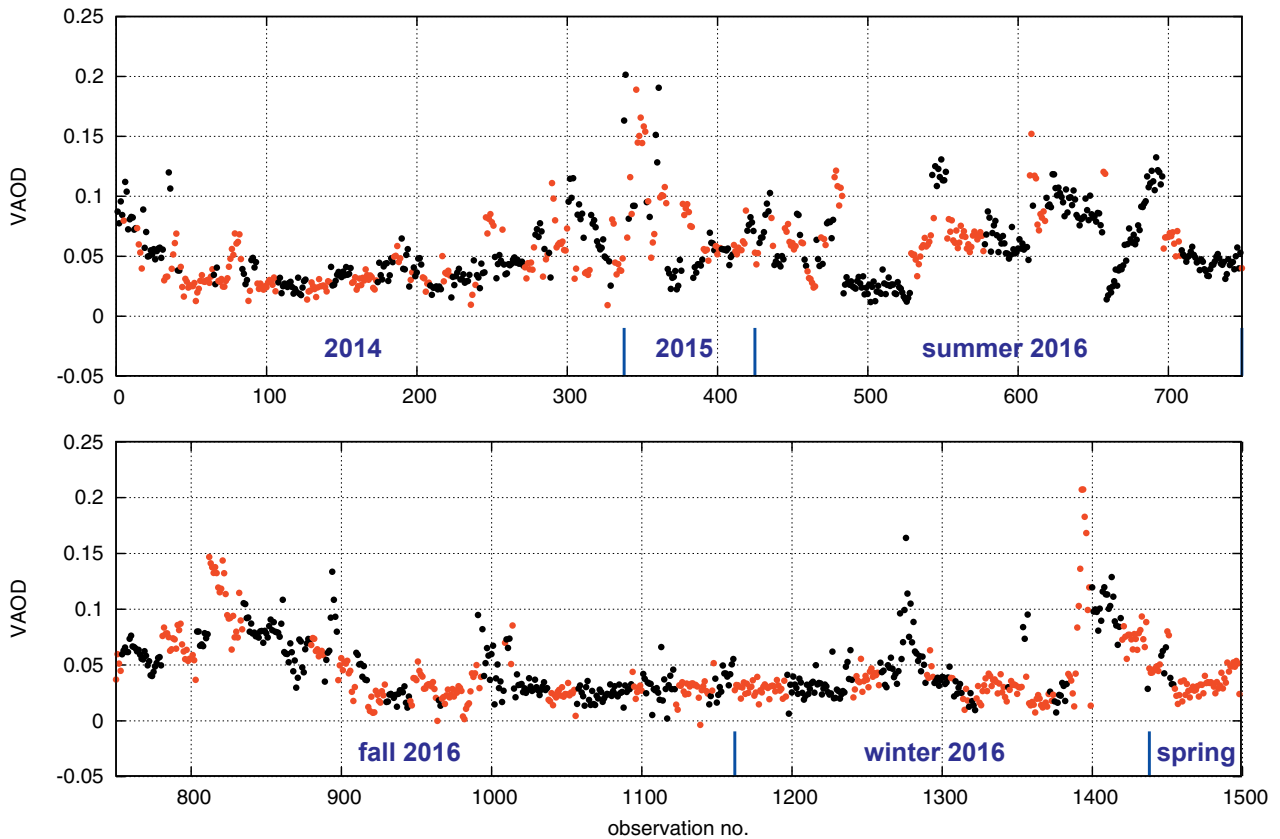
Figure 2. Time series of VAOD measurements taken by the Auger FRAM telescope located near Malargue, Argentina from 03/2014 to 11/2016. Each points represents one scan in altitude from 30 degrees elevation to the horizon in at least five 30s exposures. Consecutive points of the same color were taken during the same night, but there can be many nights skipped due to weather or hardware issues for each color change.
