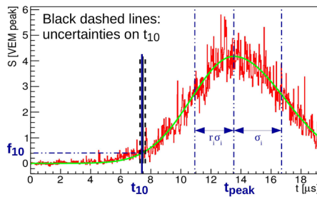
Figure 3. A typical long-lasting signal perfectly described by an asymmetric Gaussian distribution. The start time of the signal, indicated by the full blue line, is the time corresponding to the 10% of the fit function’s peak value.
