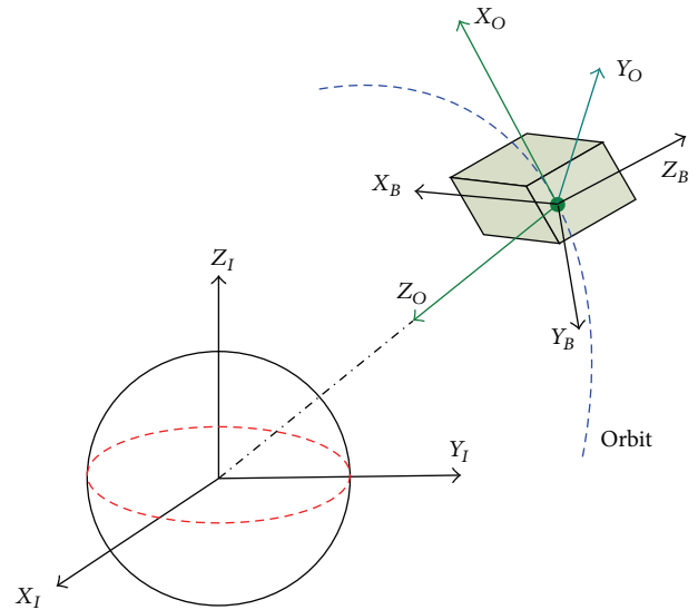
FIGURE 1: Definition of the coordinate reference frames.
