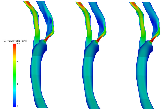
Fig. 8: Magnitude of the mean velocity vector as computed by the RANS models at \tau = 0.1s : k - k_L - \omega model (left), k - \epsilon model (center), k - \omega model (right). Quantities are plotted in the mid-plane of the carotid bifurcation. By comparison with fig. 5 (left), the transitional model is seen to be much better at reproducing the complex flow pattern in the post-stenotic region after the jet impacts the vessel wall.
