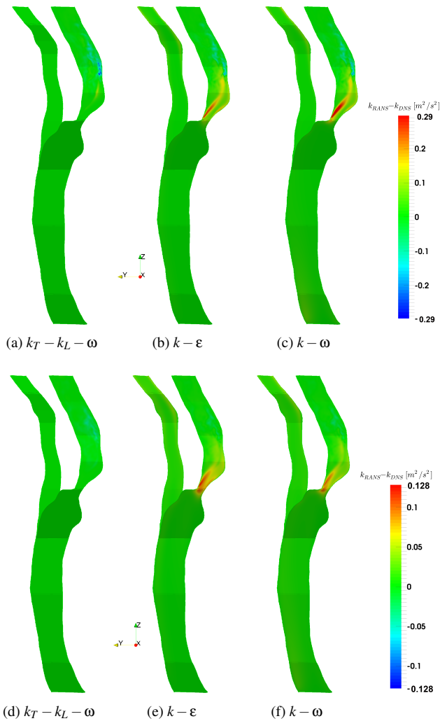
Fig. 9: Difference k_{RANS} - k_{DNS} between the turbulent kinetic energy k_{RANS} predicted by the RANS models and the same quantity k_{DNS} computed by the DNS, shown at the mid plane of the artery bifurcation. Top: \tau = 0.1s ; bottom: \tau = 0.2s . The transitional model (left) provides significantly better results overall, especially in the important region immediately downstream of the stenosis, where the two-equation models significantly overestimate the level of turbulent fluctuations.
