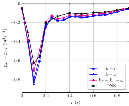
Fig. 12: Temporal evolution of the difference p_{av} - p_{ext} between the section-averaged pressure p_{av} over the section B–B, as identified in fig. 1, and the external pressure p_{ext} . The negative pressure peak at \tau = 0.1 s is overestimated by all models, but the transitional model is significantly more accurate.
