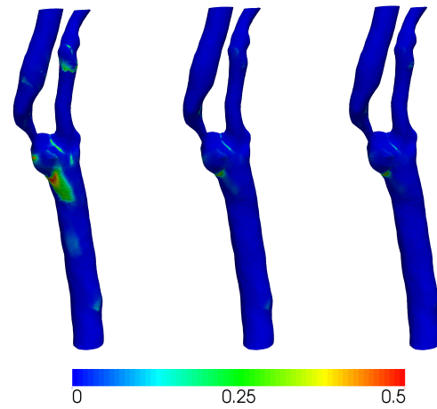
Fig. 10: OSI as computed from transitional (left), k - \epsilon (center) and k - \omega (right) RANS models. If compared with fig. 6 (right), the transitional model is seen to much better reproduce the DNS results. Two-equations RANS model predict nearly zero OSI (non-oscillatory WSS) except for small regions upstream the carotid bifurcation.
