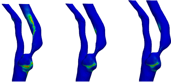
Fig. 11: OSI as computed from transitional (left), k - \epsilon (center) and k - \omega (right) RANS models: zoom on the post-stenotic region. If compared with fig. 6 (left), the transitional model predicts oscillations in the post-stenotic region in accordance with the DNS result, but the complex pattern is not correctly reproduced. Two-equations RANS models significantly underestimate the extent of WSS vector oscillation in the post-stenotic region.
