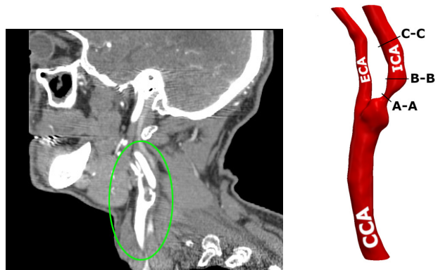
Fig. 1: Left: sagittal section of the CTA, with the carotid artery highlighted in white by the contrast medium. Right: the vessel geometry employed in the present work, showing the stenosed section A-A.
