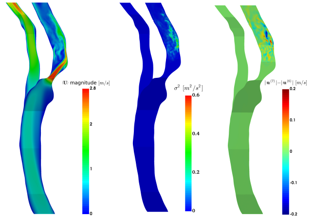
Fig. 5: Phase-averaged magnitude of the velocity vector (left) and its temporal variance (center) at \tau = 0.1s . The ensemble average is performed over 7 cycles, and the temporal variance gives an hint of the statistical error associated to the estimate of the expected value of the mean. On the right, difference between the mean velocity field |\langle \mathbf{u} \rangle^{(7)}| obtained averaging over 7 cycles, and the same quantity obtained over 6 cycles.
