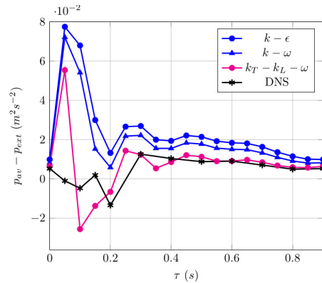
Fig. 13: Temporal evolution of the difference p_{av} - p_{ext} between the section-averaged pressure p_{av} over the section C–C, as identified in fig. 1, and the external pressure p_{ext} . The k_T - k_L - \omega points lie on the DNS curve after the systolic peak. Near the systolic peak at \tau = 0.1 s the transitional model is the only one to be not too far off the DNS values.
