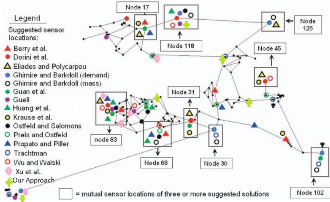
Figure 7. WDN network (BWSN) and alternative sensor nodes location solutions.
