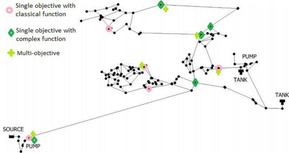
Figure 5. Optimal sensor node locations in the WDN network (BWSN), for the three cases of single-objective F_1, F_2 and bi-objective F optimization which are located in the inner and the outer sides of the network
