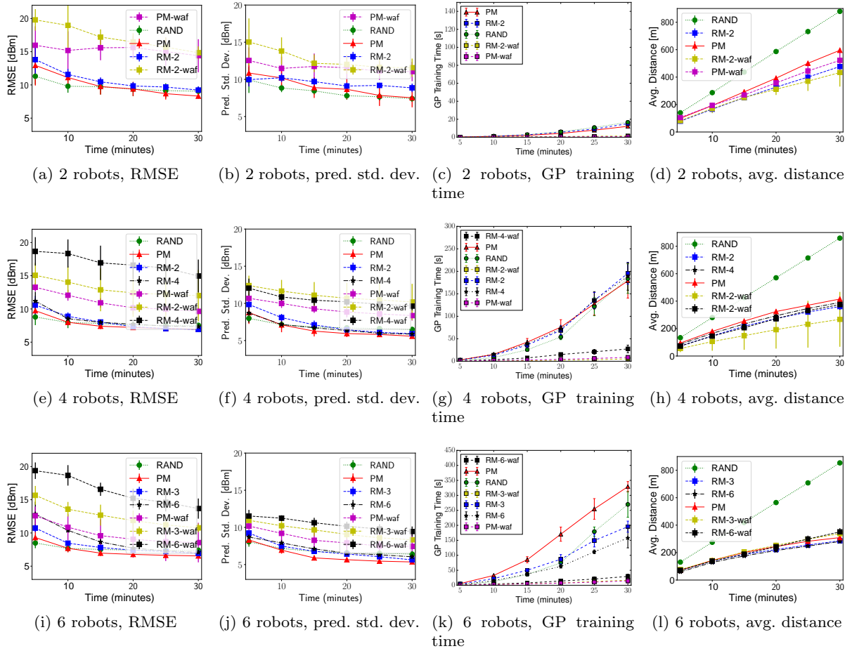
Fig. 7: Simulation experiments, Office environment, zero-mean GP.
