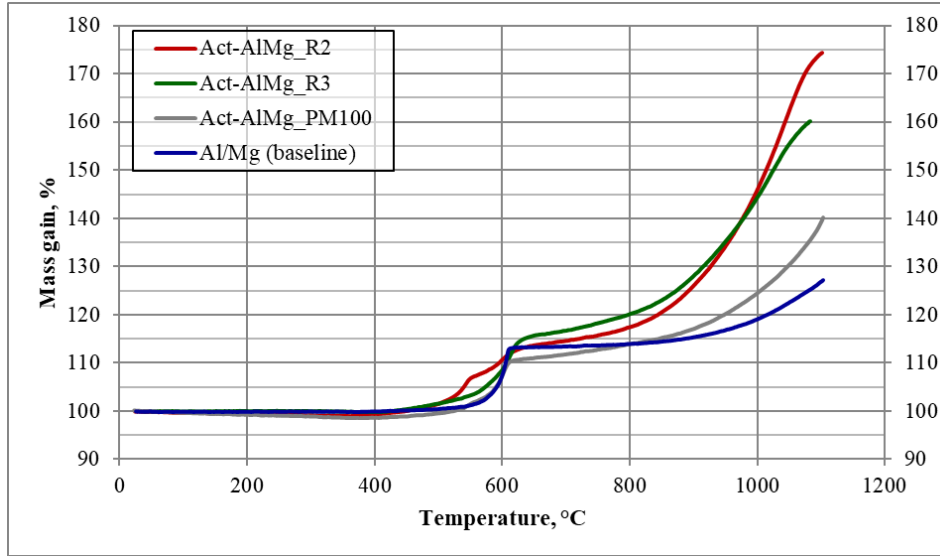
Figure 3. TG traces for the tested samples.
