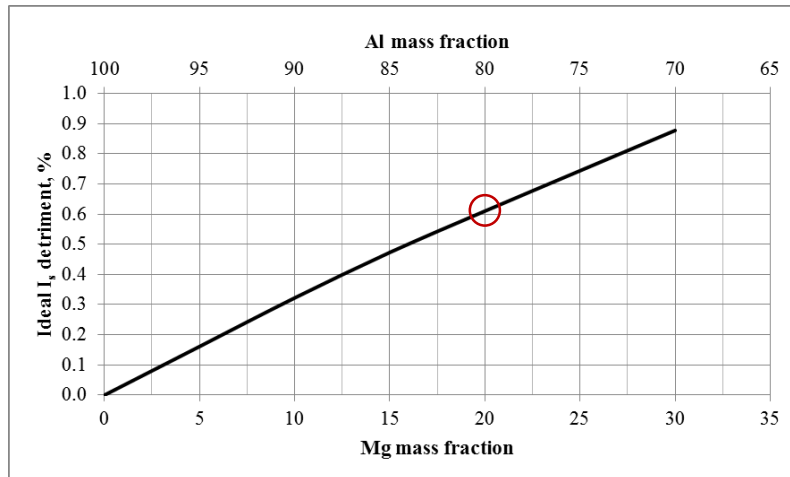
Figure 1. Detriment of the ideal specific impulse caused by the addition of Mg/Al mixtures in HTPB/AN-based SPs under reference conditions. The red circle indicates the design point.
