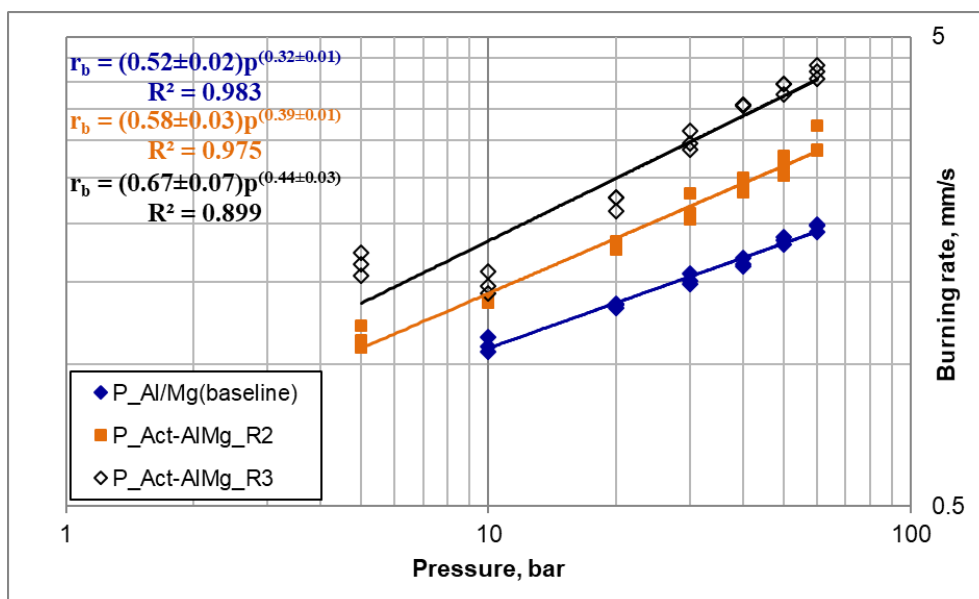
Figure 4. Burning rate of solid rocket propellants loaded with AN and activated Al/Mg powders.
