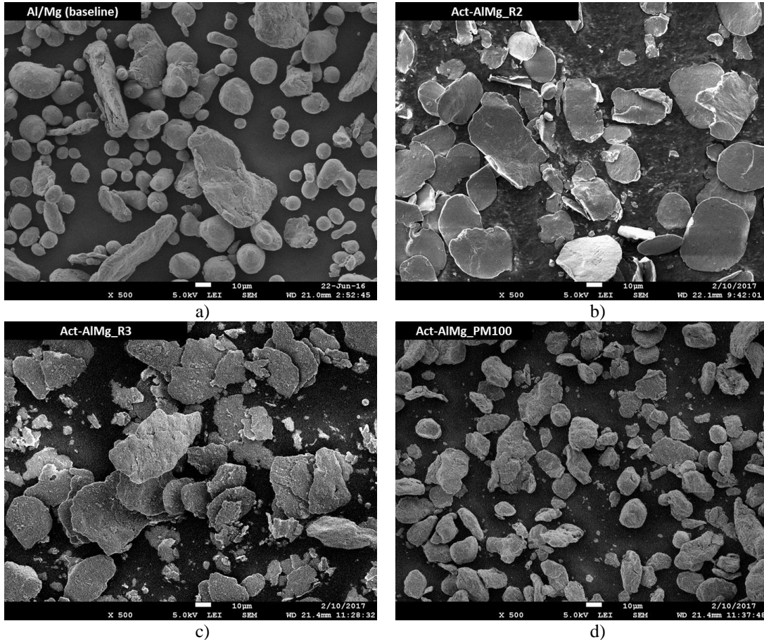
Figure 2. SEM images of activated powders. The virgin mixture and a powder activated through a standard technique (Act-AlMg_PM100) are reported for comparison.
