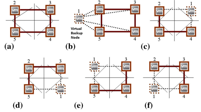
Fig. 5 Basic cuts, post-disaster cuts, and one VM backup location per CN. a CN with basic cuts, b CN with one VM backup location and c–f extended cuts for any replacement
