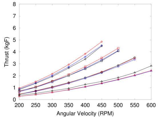
(b) Yun et al. T vs. \Omega .
