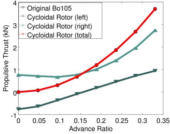
(a) Propulsive thrust.
