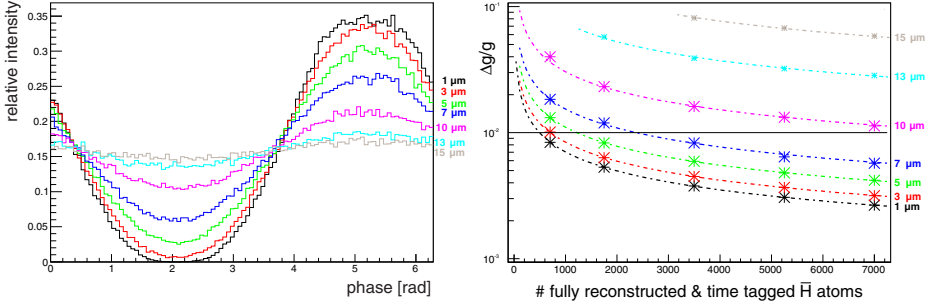
Fig. 2 Left : Simulated distribution of reconstructed annihilation vertices on the free-fall detector over one grating period for vertex resolutions between 1 and 15 \mu\text{m} for an antihydrogen beam with a velocity of 700 m/s. The contrast of the shadow-like image increases with improved vertex resolution. Right : Simulation of the relative precision on \bar{g} vs. the number of fully reconstructed and time tagged antihydrogen atoms for vertex resolutions between 1 and 15 \mu\text{m} . The horizontal black line indicates a 1% relative error on \bar{g} [5]
