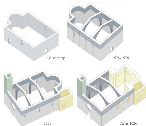
Figure 3. St. Antonio Oratory main evolution phases layouts.
